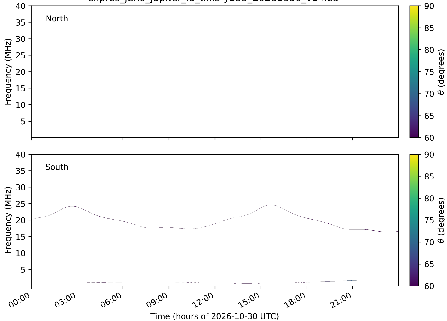
expres_juno_jupiter_io_txka-y235_20261030_v14.cdf
