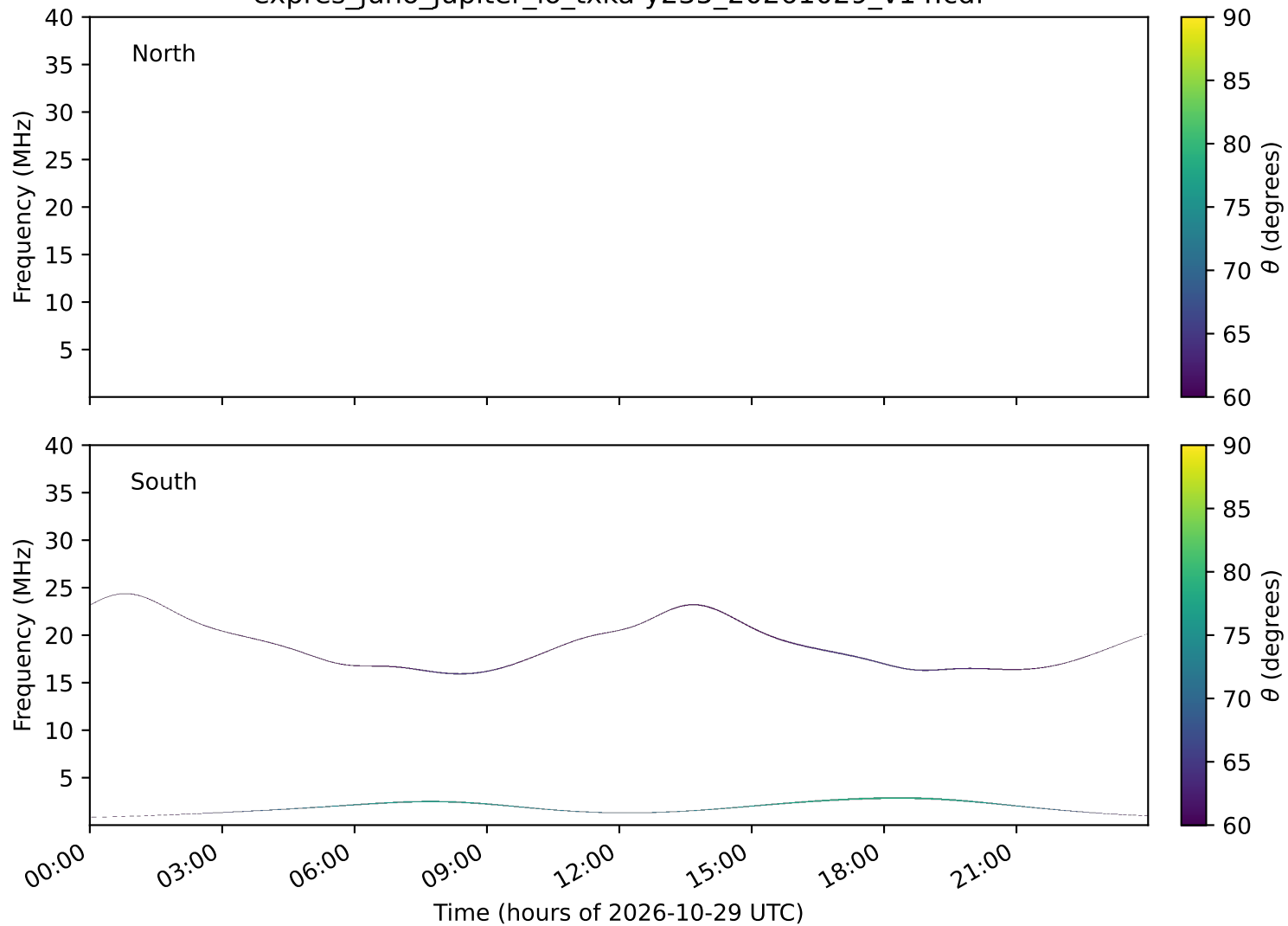
expres_juno_jupiter_io_txka-y235_20261029_v14.cdf
