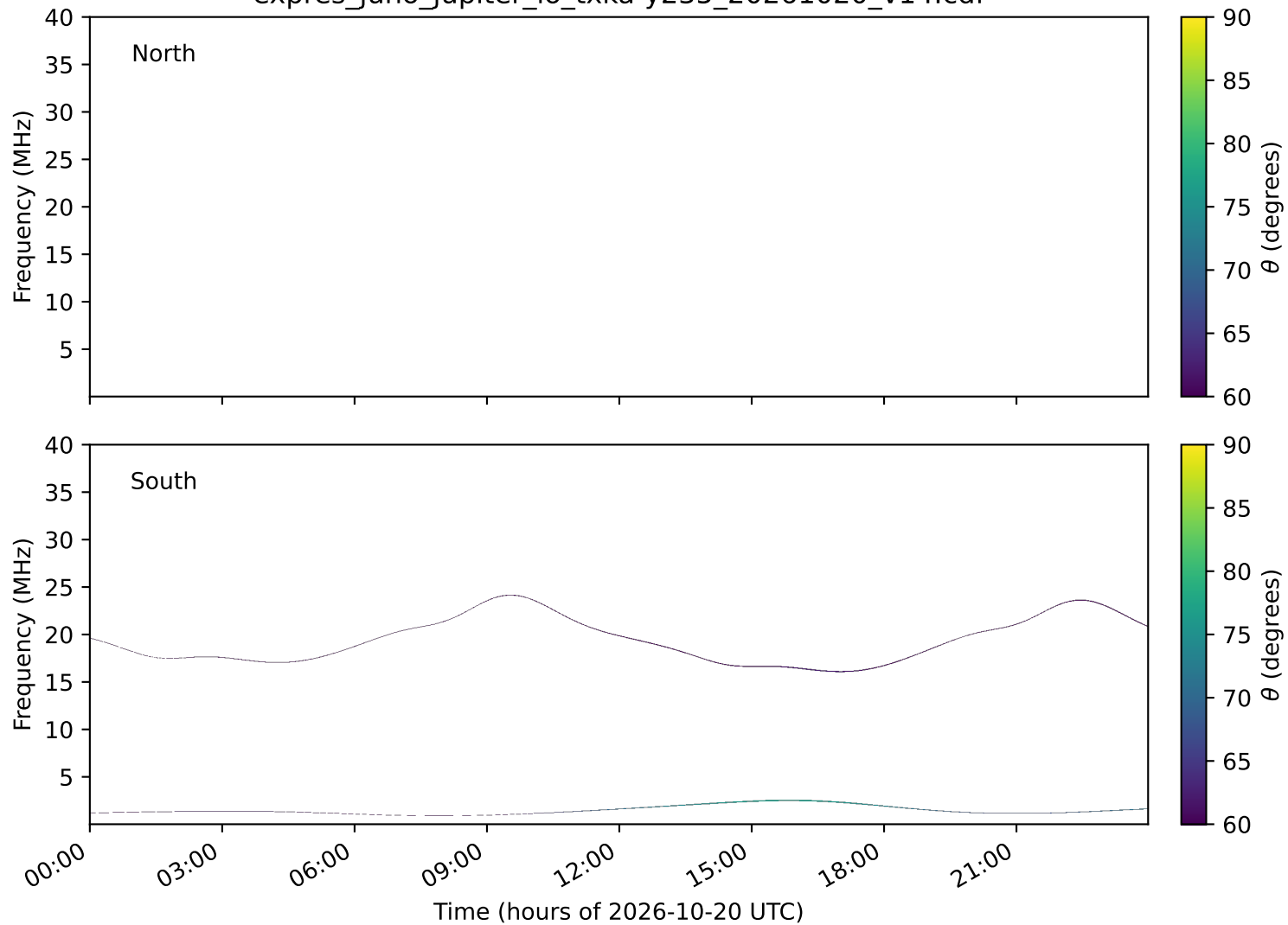
expres_juno_jupiter_io_txka-y235_20261020_v14.cdf
