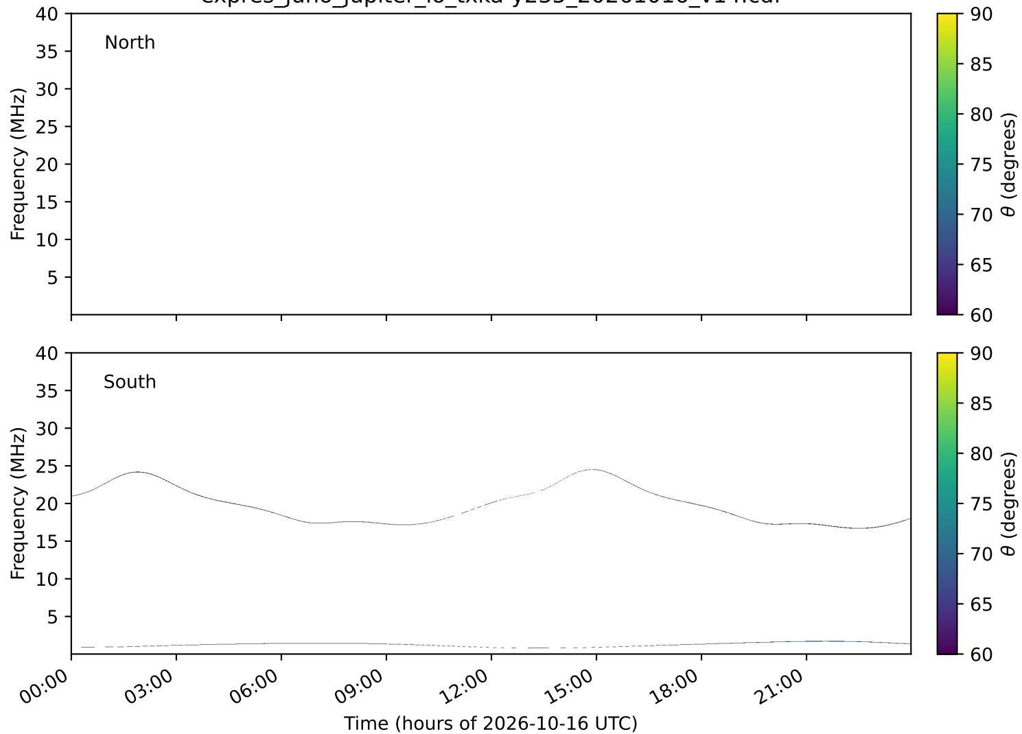
expres_juno_jupiter_io_txka-y235_20261016_v14.cdf
