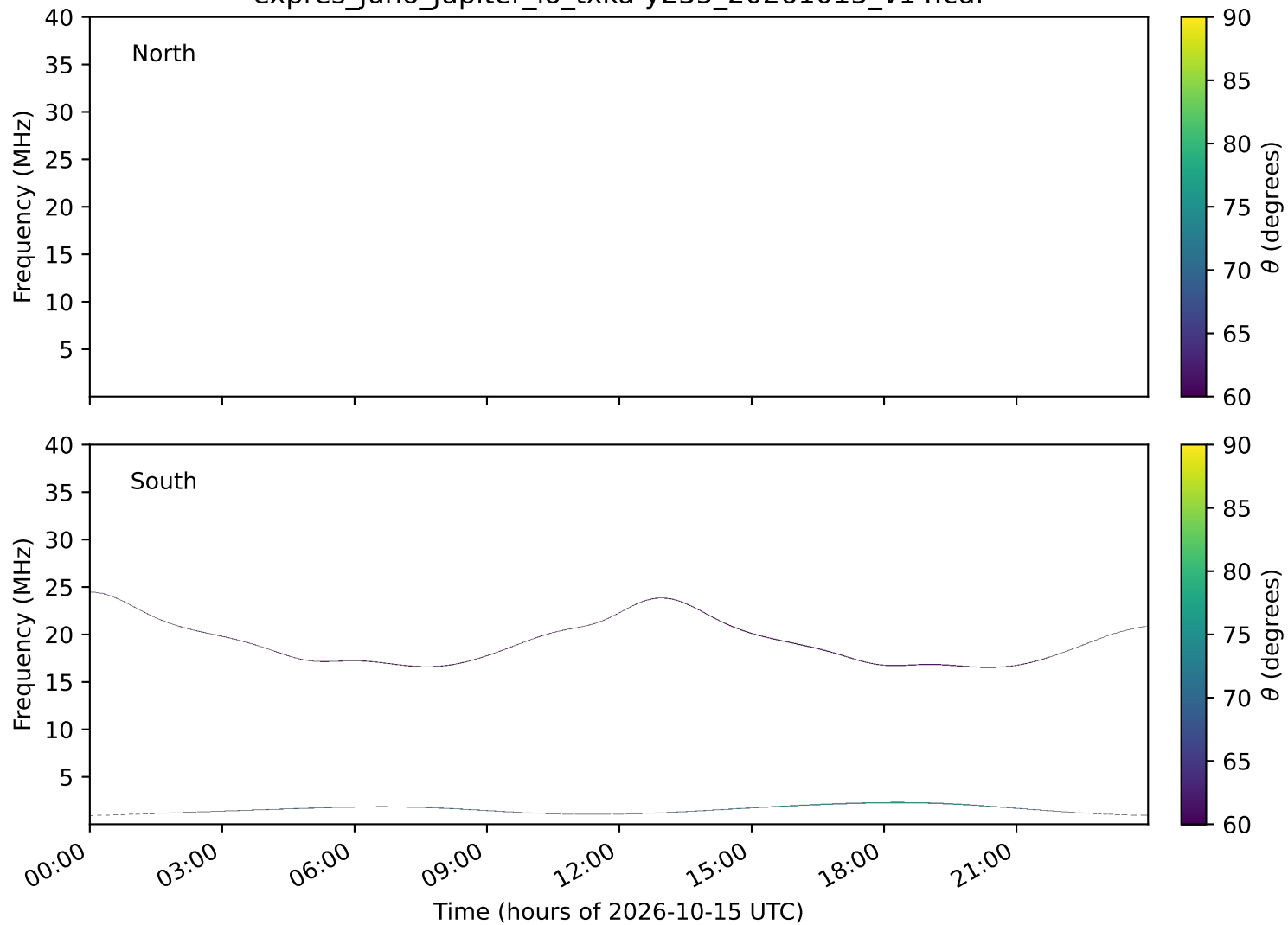
expres_juno_jupiter_io_txka-y235_20261015_v14.cdf
