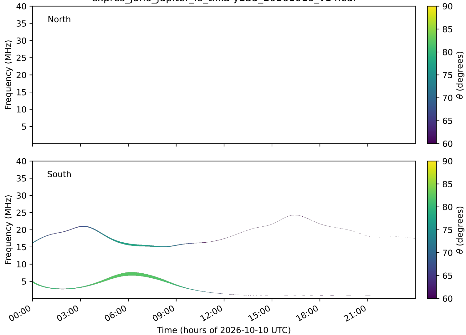
expres_juno_jupiter_io_txka-y235_20261010_v14.cdf
