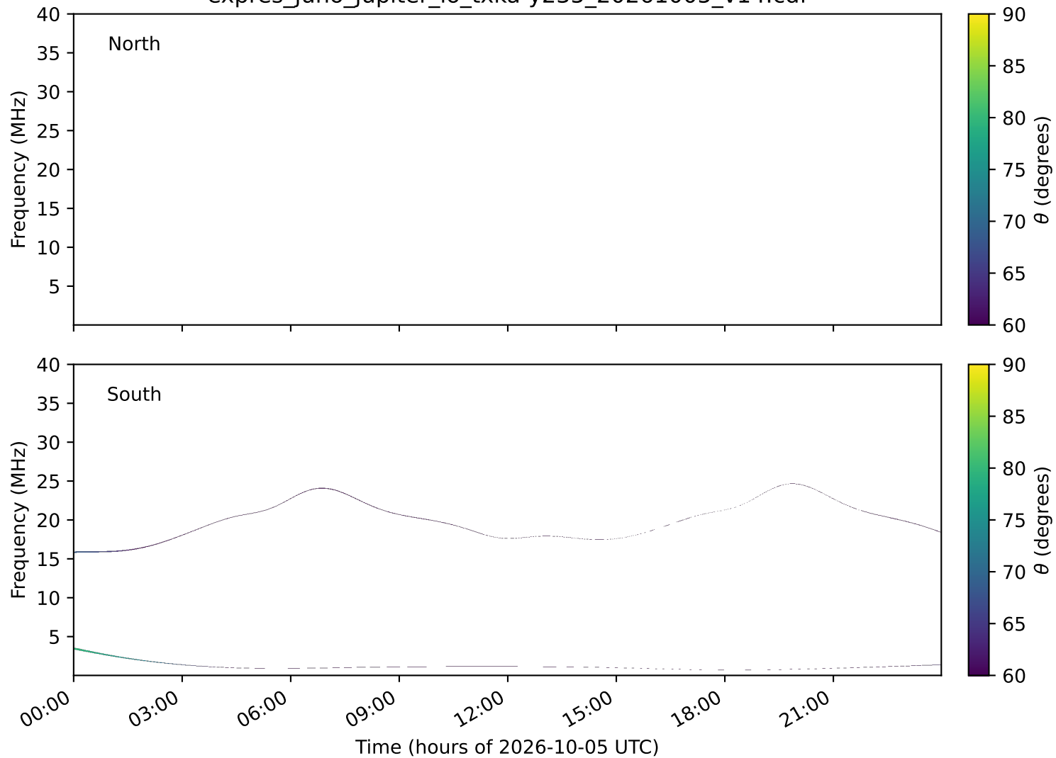
expres_juno_jupiter_io_txka-y235_20261005_v14.cdf
