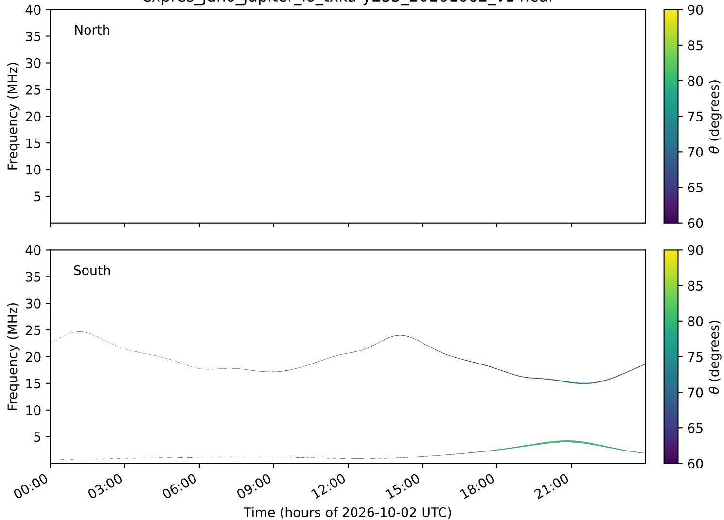
expres_juno_jupiter_io_txka-y235_20261002_v14.cdf
