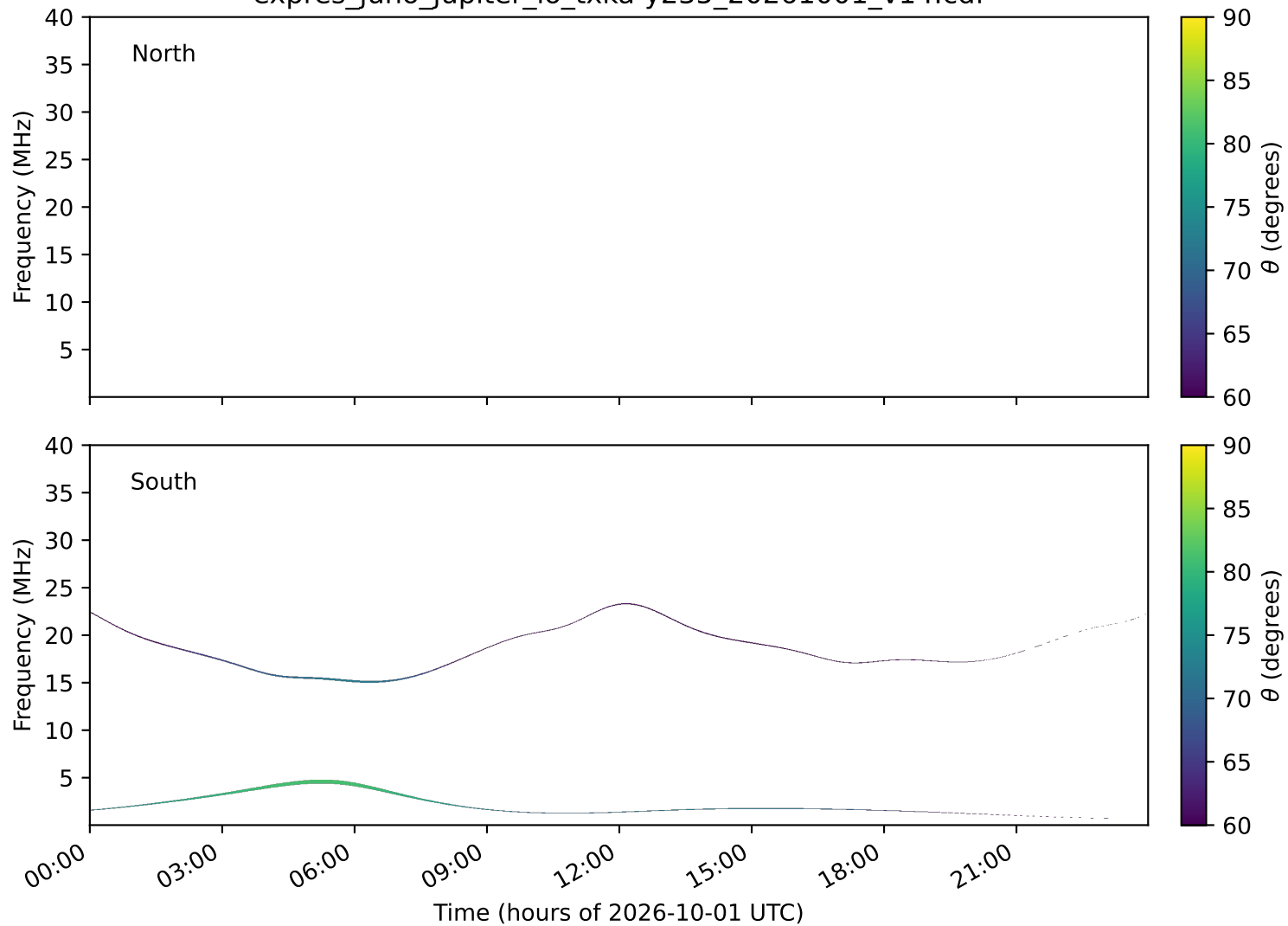
expres_juno_jupiter_io_txka-y235_20261001_v14.cdf
