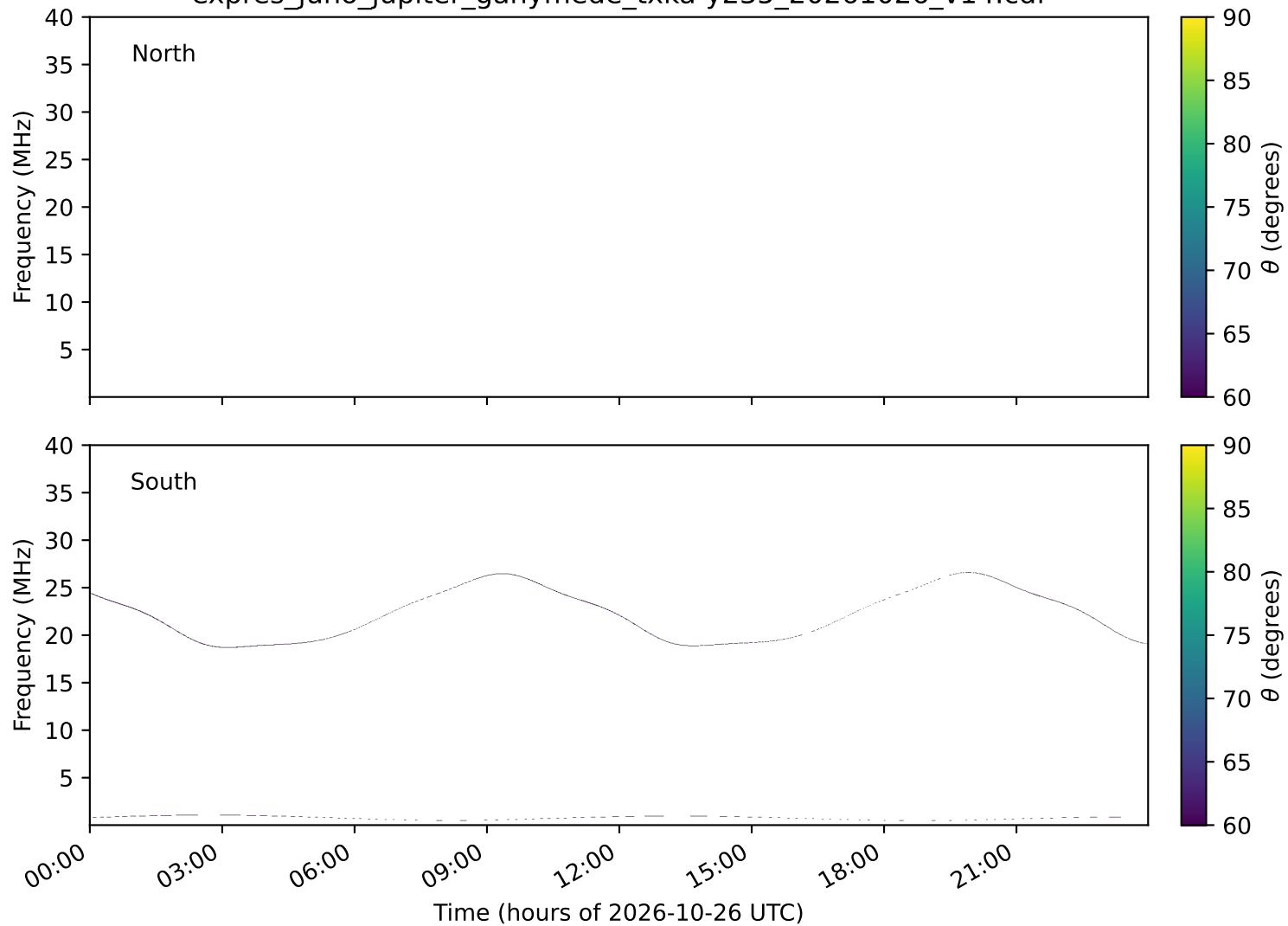
expres_juno_jupiter_ganymede_txka-y235_20261026_v14.cdf
