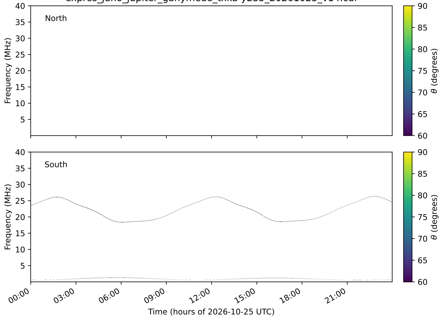
expres_juno_jupiter_ganymede_txka-y235_20261025_v14.cdf
