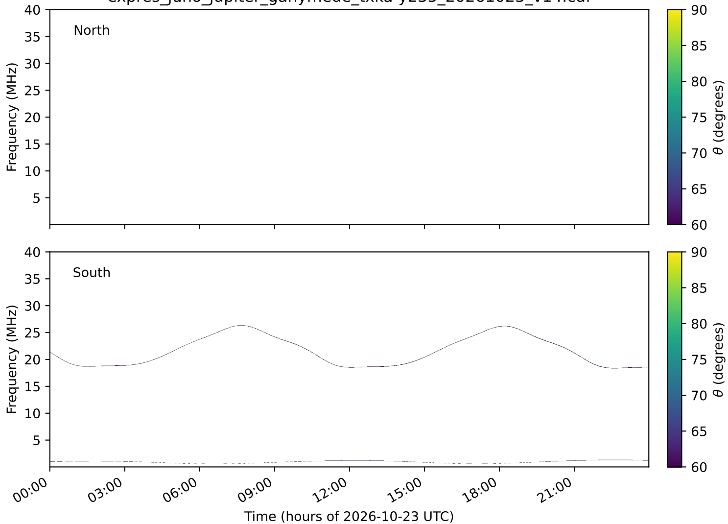
expres_juno_jupiter_ganymede_txka-y235_20261023_v14.cdf
