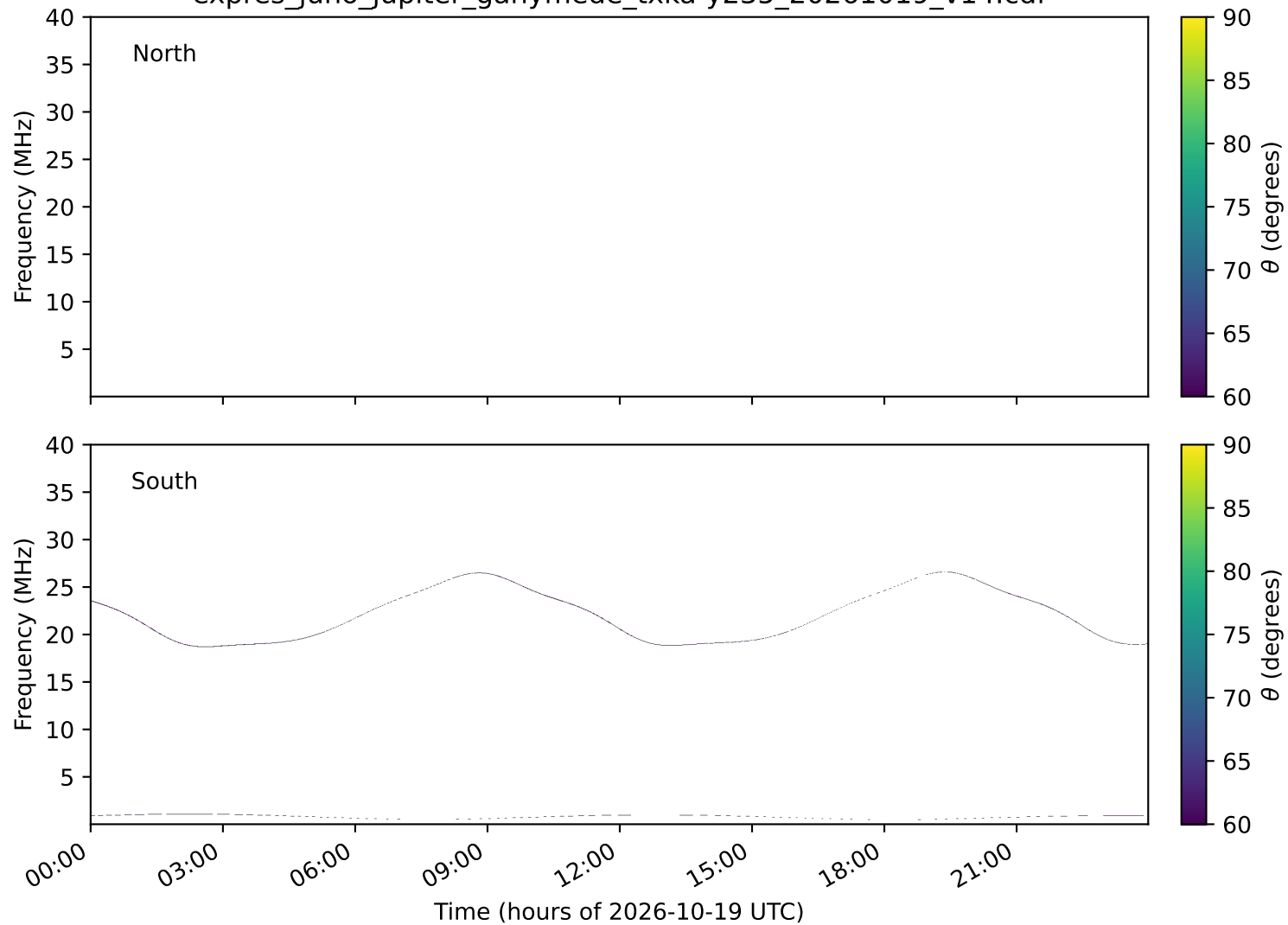
expres_juno_jupiter_ganymede_txka-y235_20261019_v14.cdf
