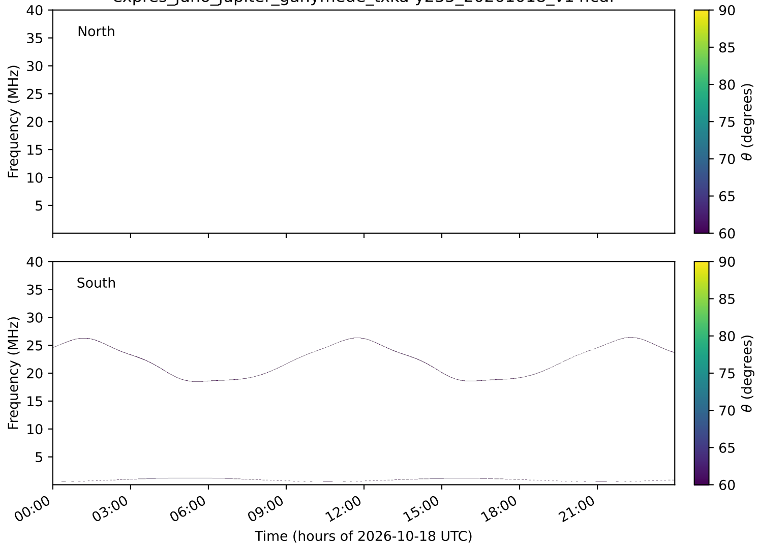
expres_juno_jupiter_ganymede_txka-y235_20261018_v14.cdf
