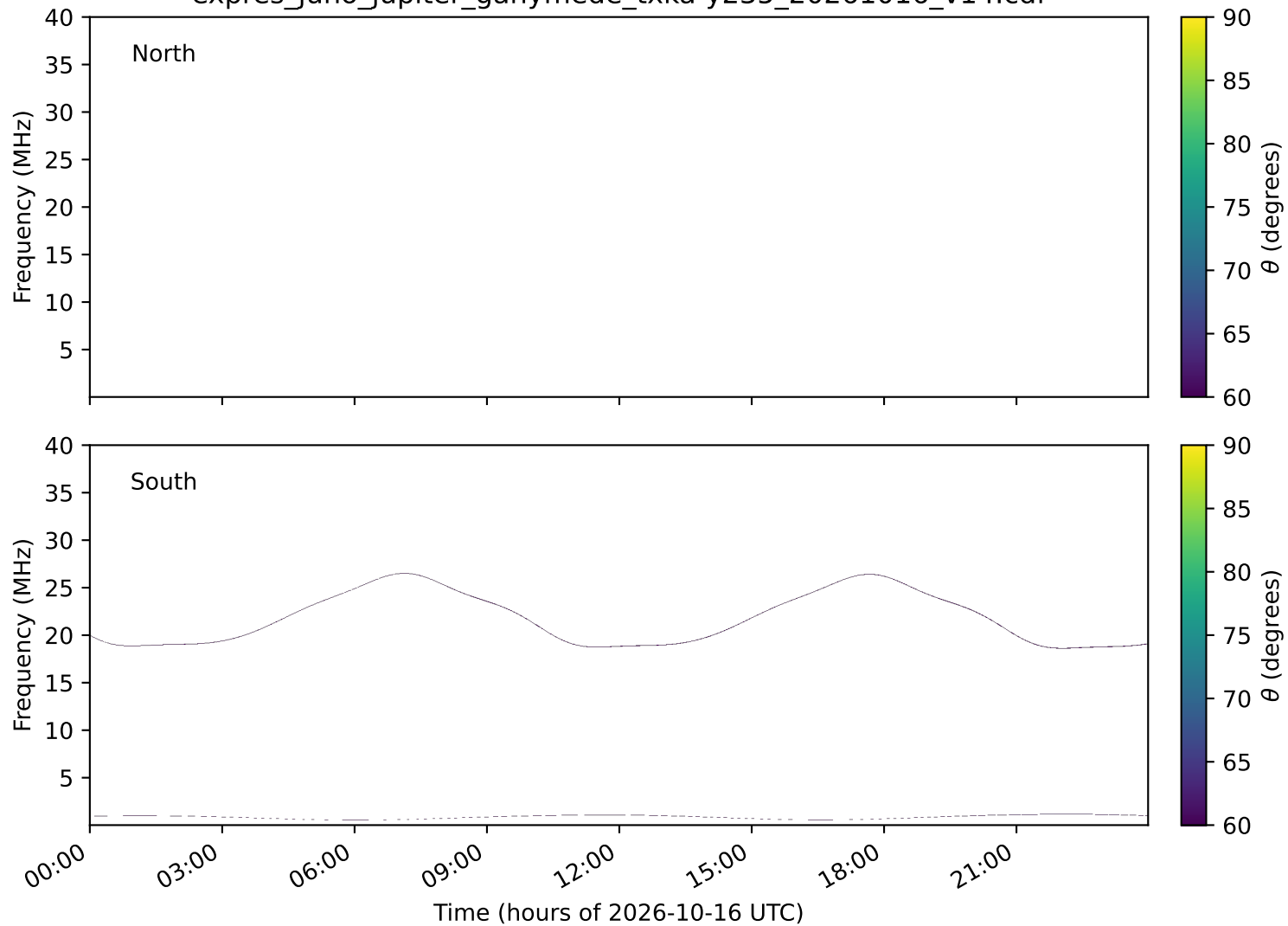
expres_juno_jupiter_ganymede_txka-y235_20261016_v14.cdf
