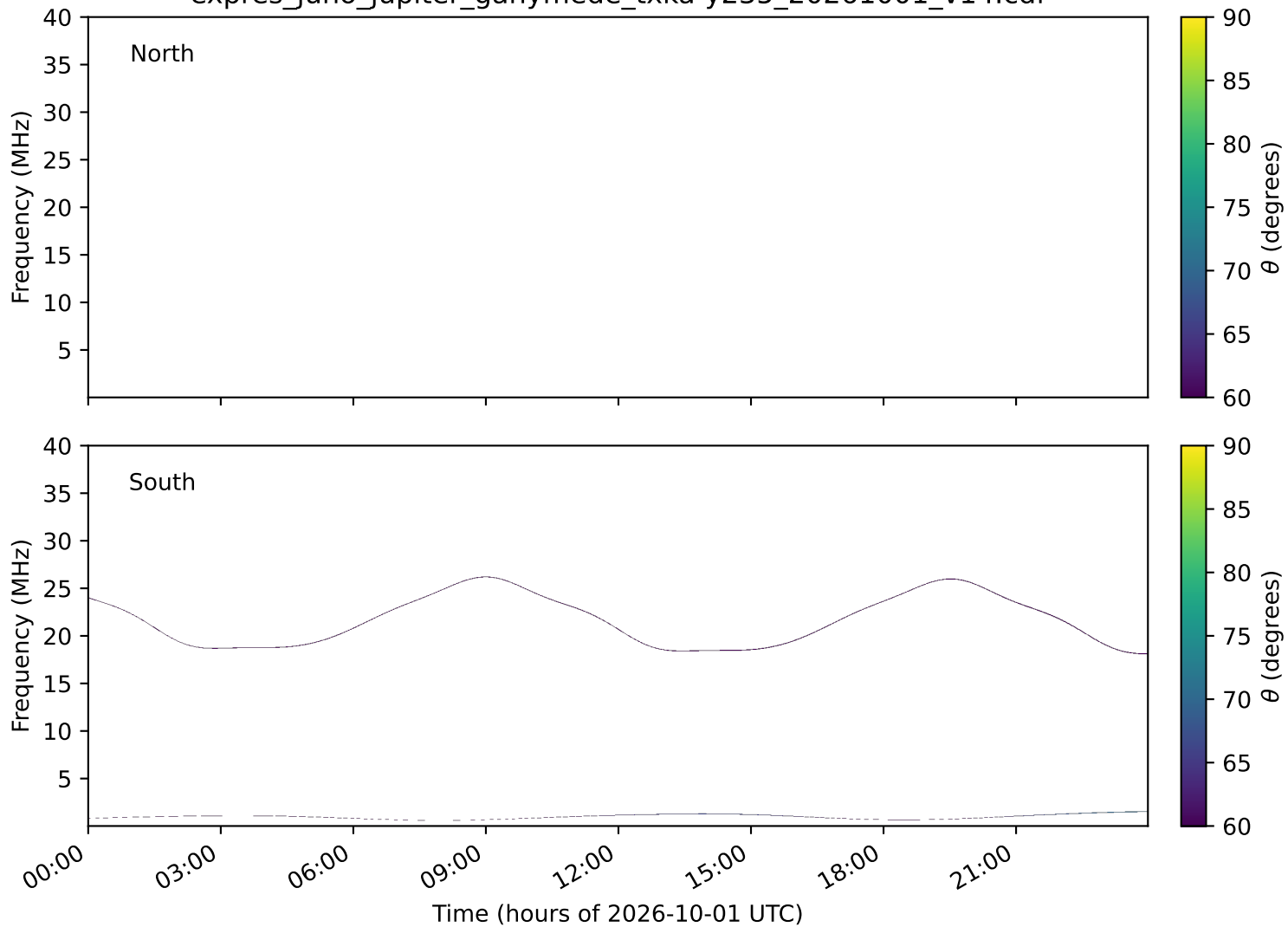
expres_juno_jupiter_ganymede_txka-y235_20261001_v14.cdf
