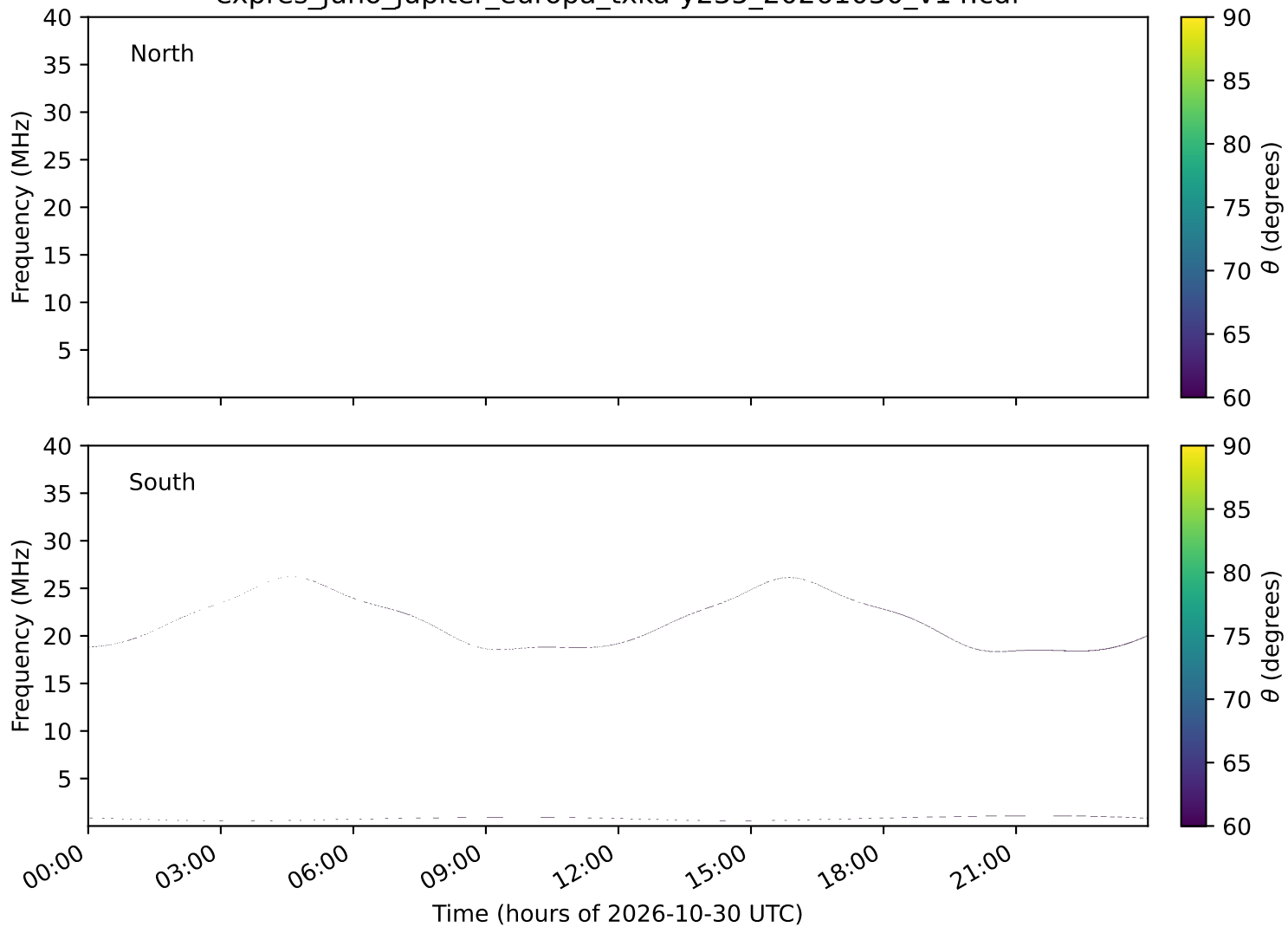
expres_juno_jupiter_europa_txka-y235_20261030_v14.cdf
