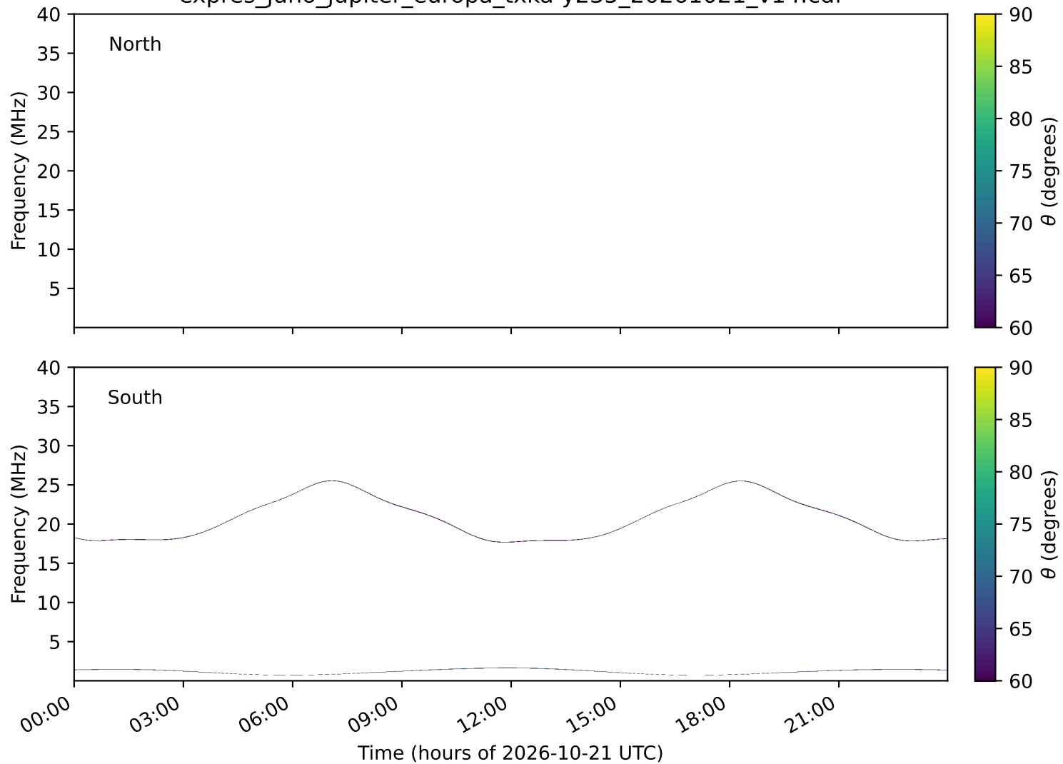
expres_juno_jupiter_europa_txka-y235_20261021_v14.cdf
