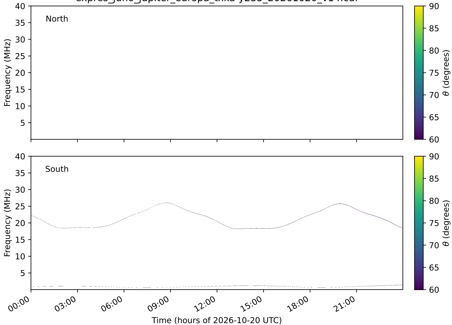
expres_juno_jupiter_europa_txka-y235_20261020_v14.cdf
