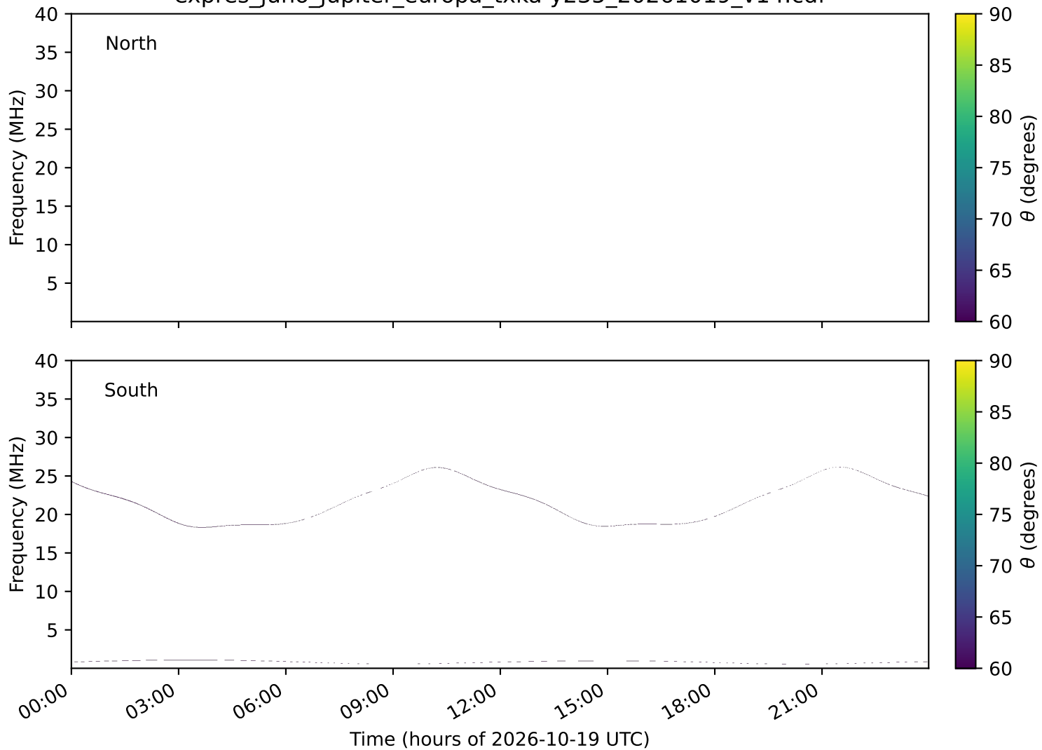
expres_juno_jupiter_europa_txka-y235_20261019_v14.cdf
