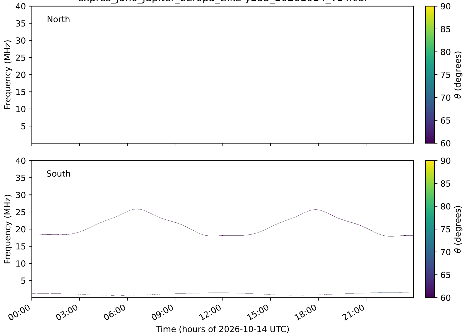
expres_juno_jupiter_europa_txka-y235_20261014_v14.cdf
