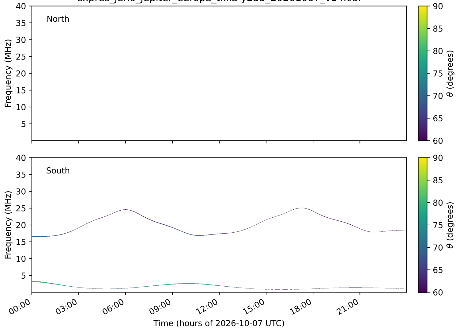
expres_juno_jupiter_europa_txka-y235_20261007_v14.cdf
