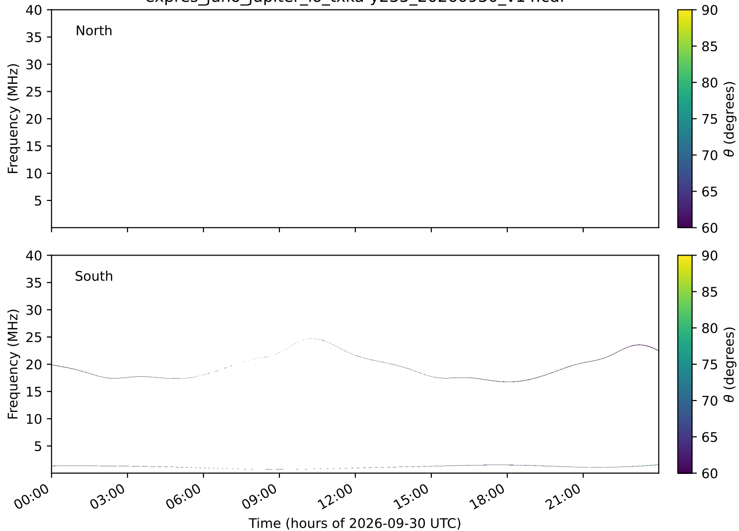
expres_juno_jupiter_io_txka-y235_20260930_v14.cdf
