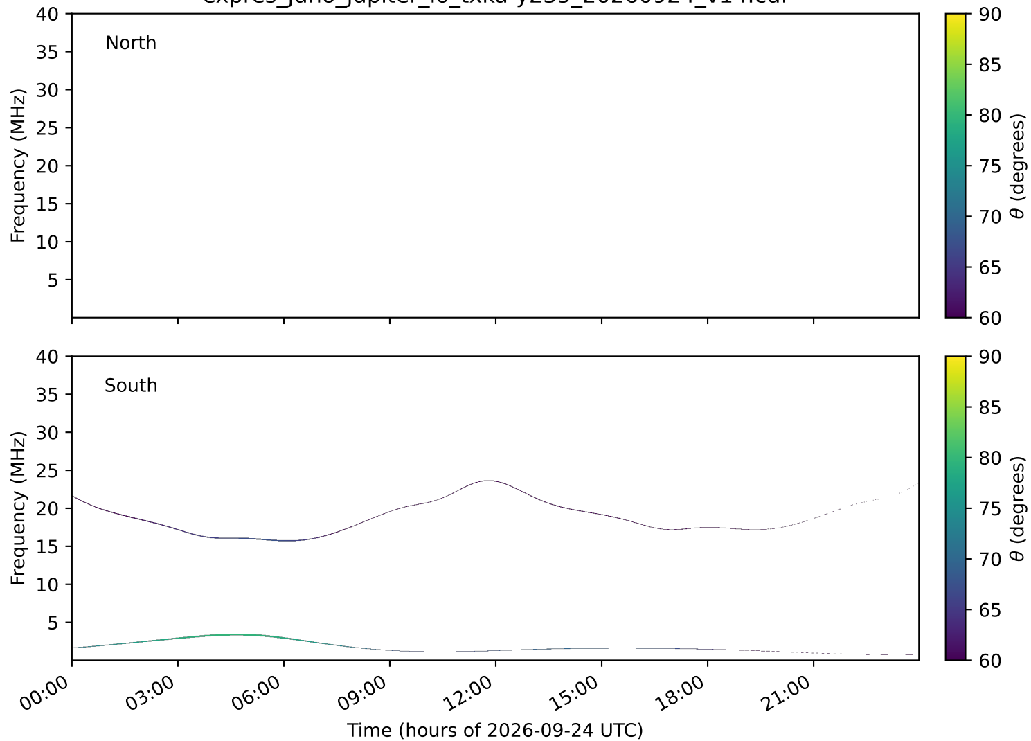
expres_juno_jupiter_io_txka-y235_20260924_v14.cdf
