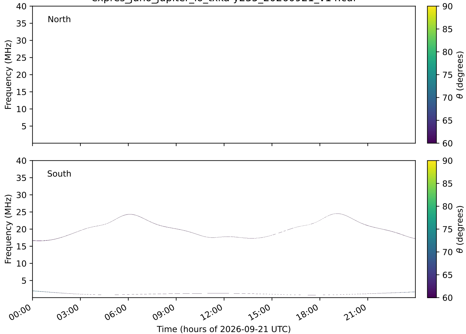
expres_juno_jupiter_io_txka-y235_20260921_v14.cdf
