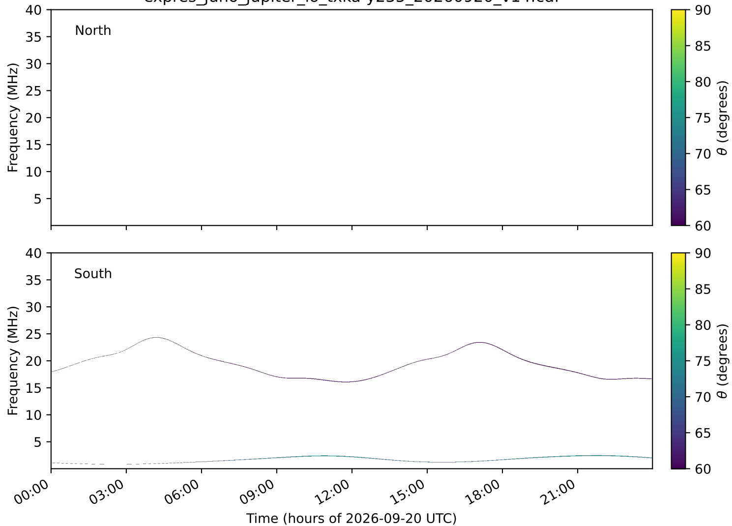
expres_juno_jupiter_io_txka-y235_20260920_v14.cdf
