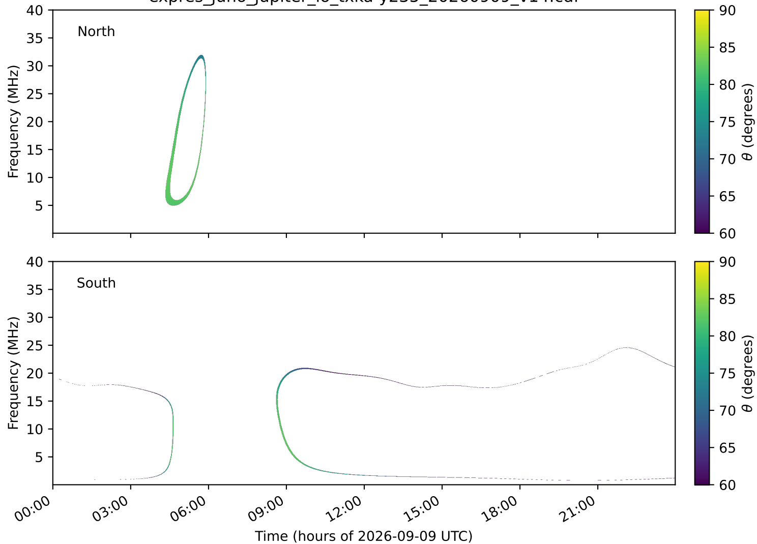
expres_juno_jupiter_io_txka-y235_20260909_v14.cdf
