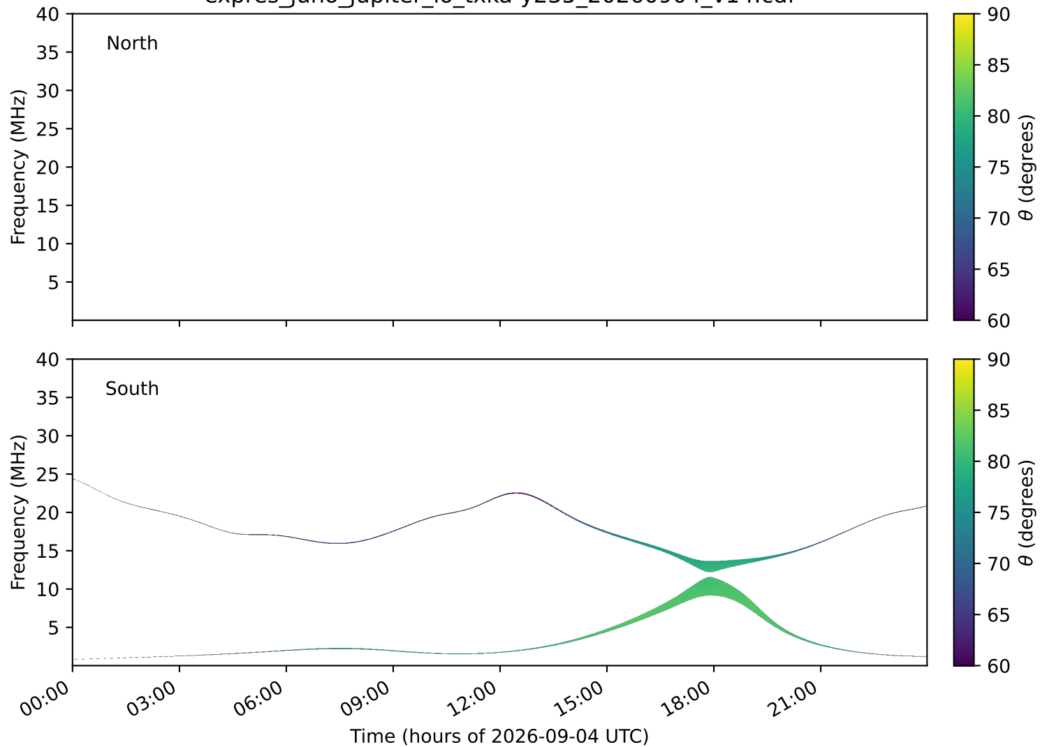
expres_juno_jupiter_io_txka-y235_20260904_v14.cdf
