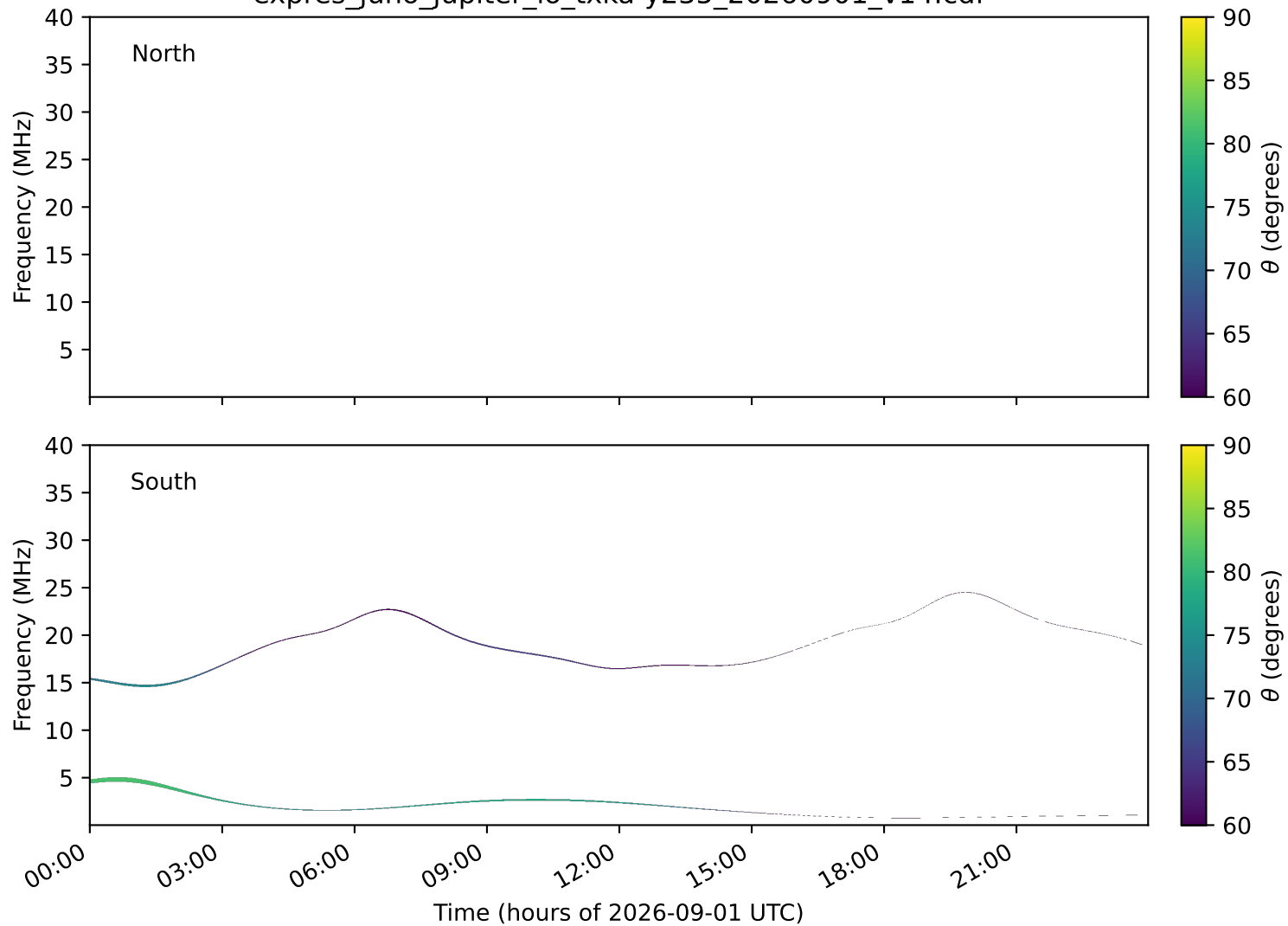
expres_juno_jupiter_io_txka-y235_20260901_v14.cdf
