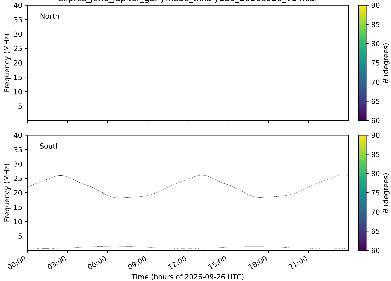
expres_juno_jupiter_ganymede_txka-y235_20260926_v14.cdf
