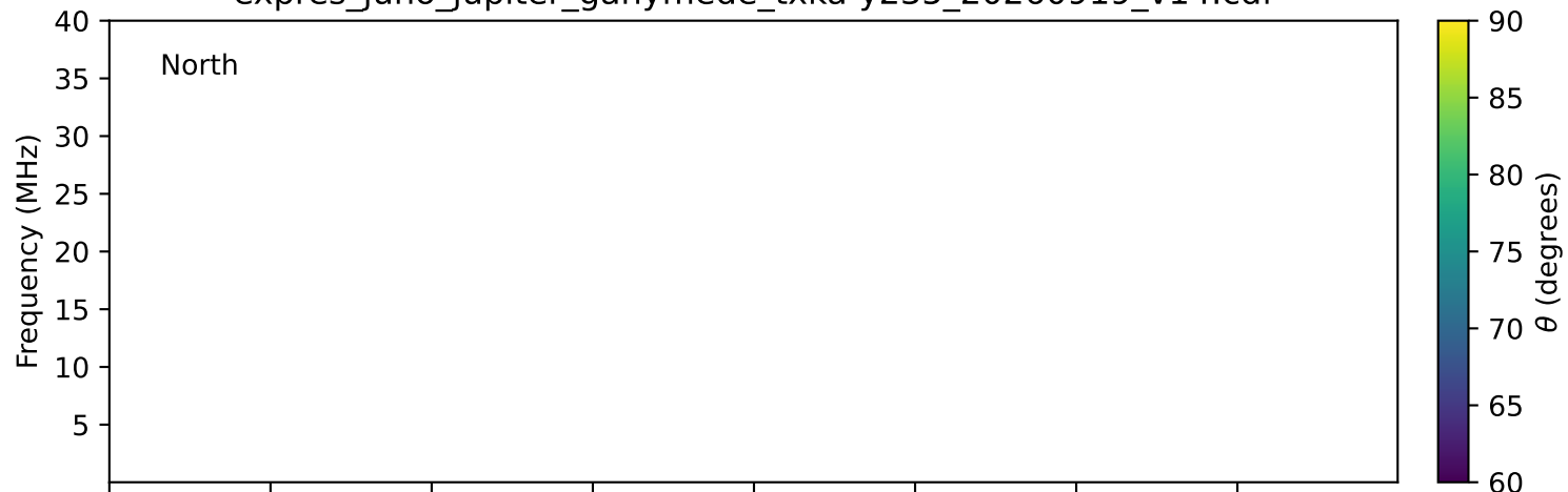
expres_juno_jupiter_ganymede_txka-y235_20260919_v14.cdf
