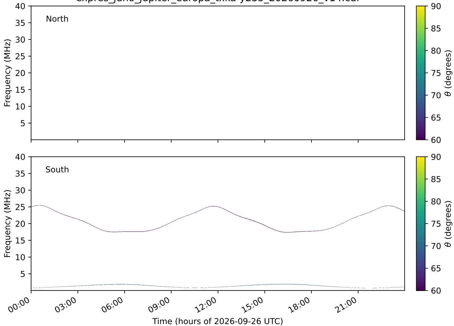
expres_juno_jupiter_europa_txka-y235_20260926_v14.cdf
