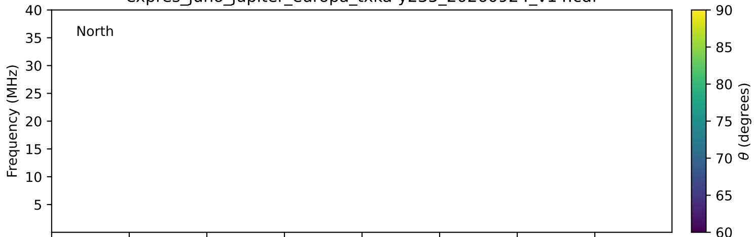
expres_juno_jupiter_europa_txka-y235_20260924_v14.cdf
