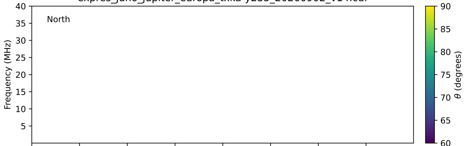
expres_juno_jupiter_europa_txka-y235_20260902_v14.cdf
