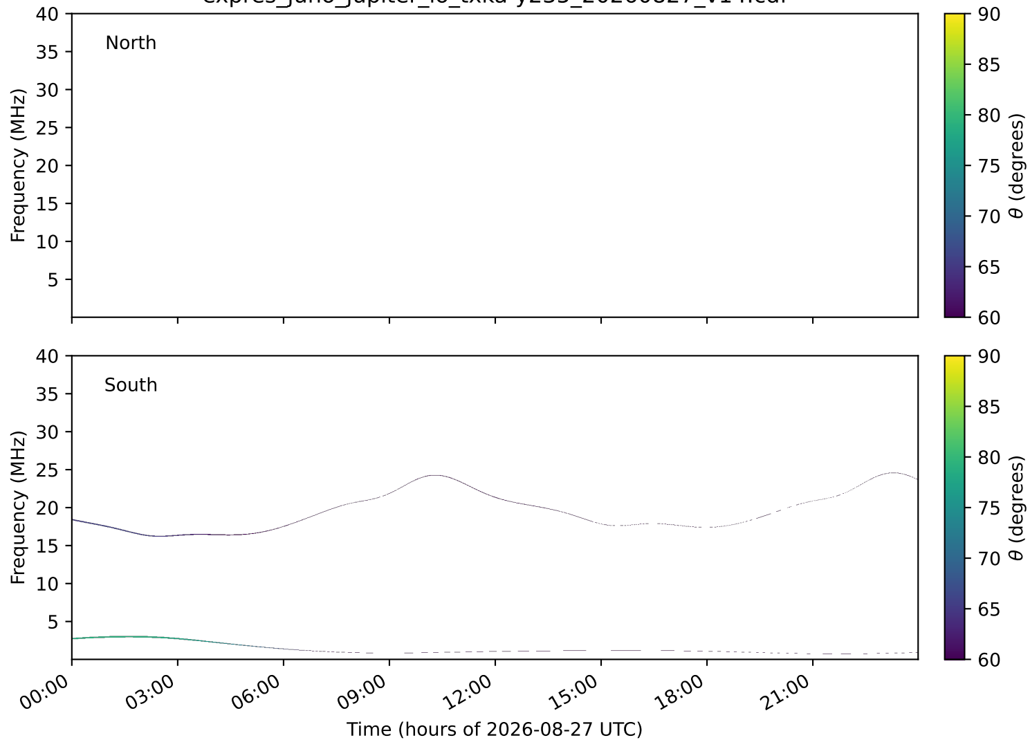
expres_juno_jupiter_io_txka-y235_20260827_v14.cdf
