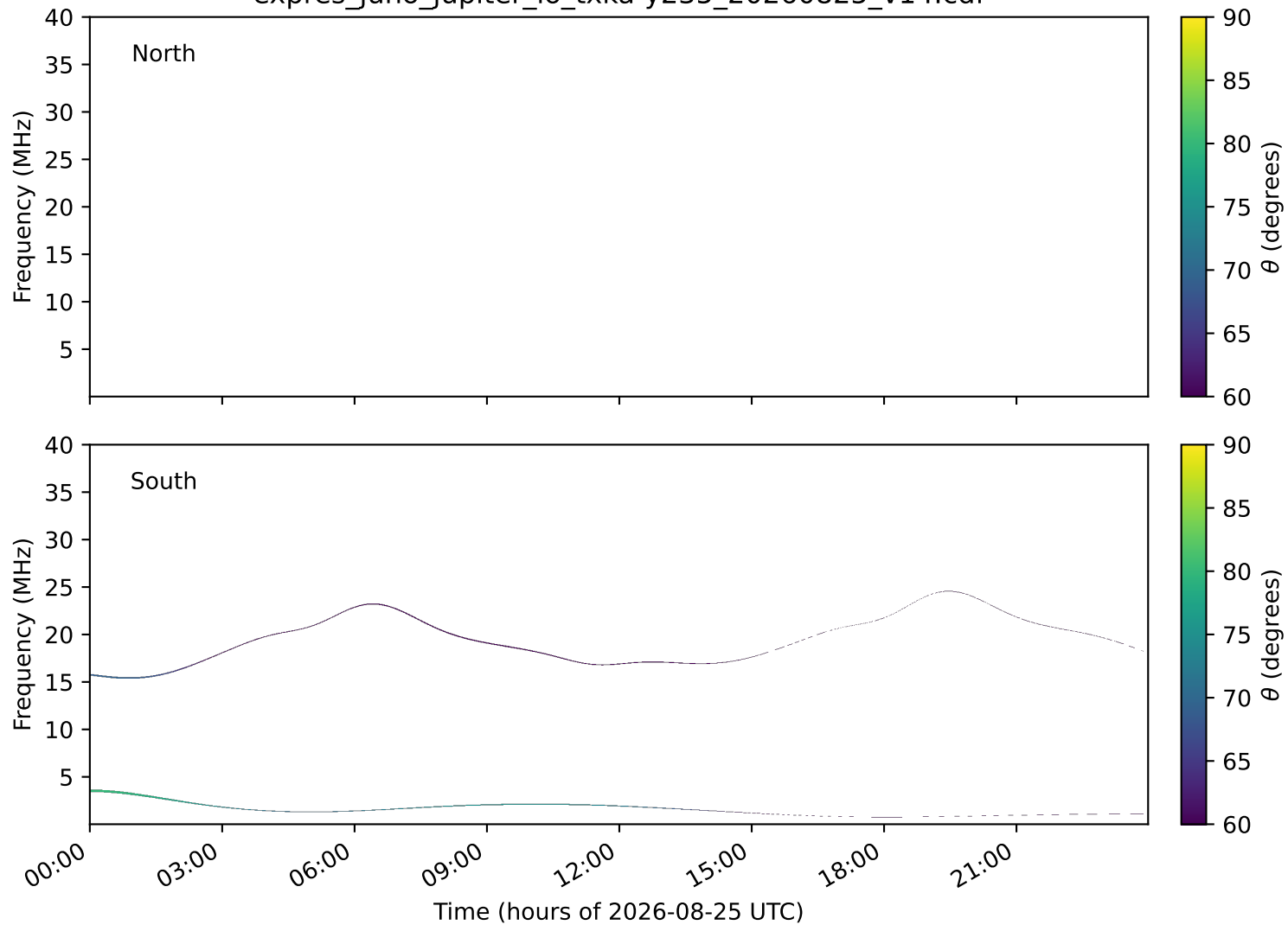
expres_juno_jupiter_io_txka-y235_20260825_v14.cdf
