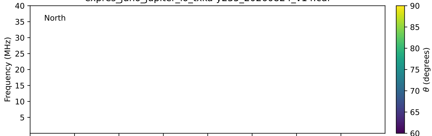
expres_juno_jupiter_io_txka-y235_20260824_v14.cdf
