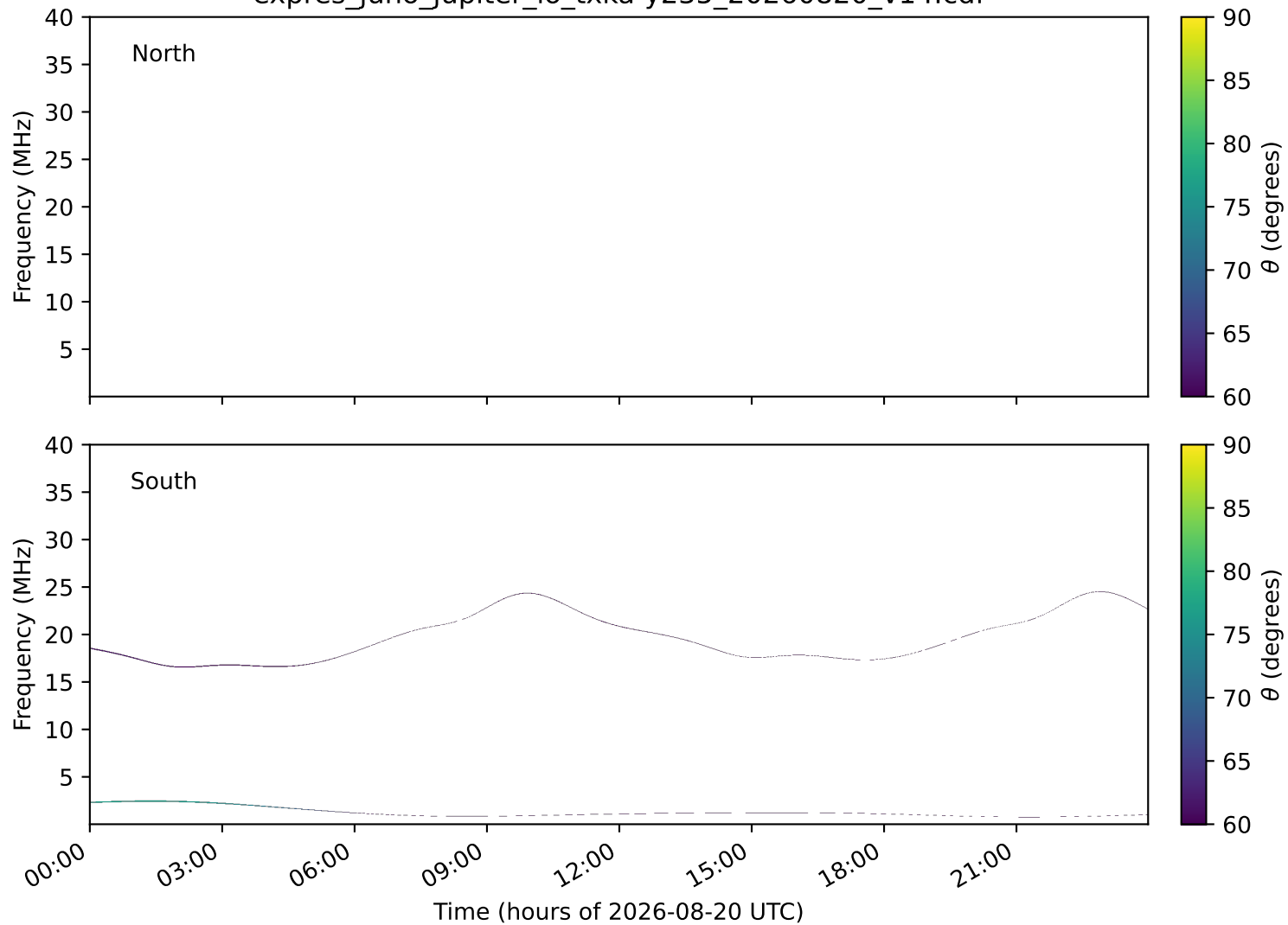
expres_juno_jupiter_io_txka-y235_20260820_v14.cdf
