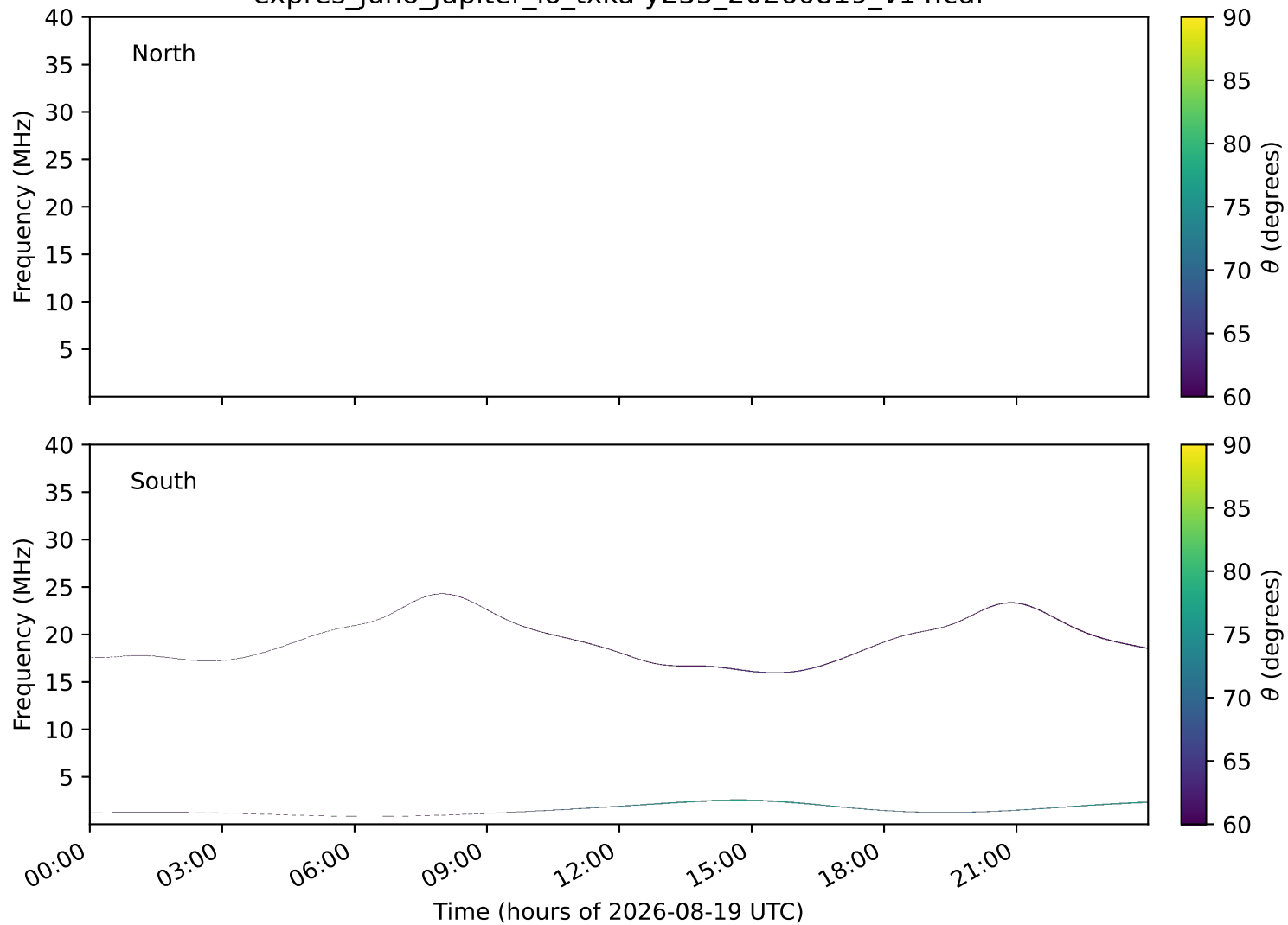
expres_juno_jupiter_io_txka-y235_20260819_v14.cdf
