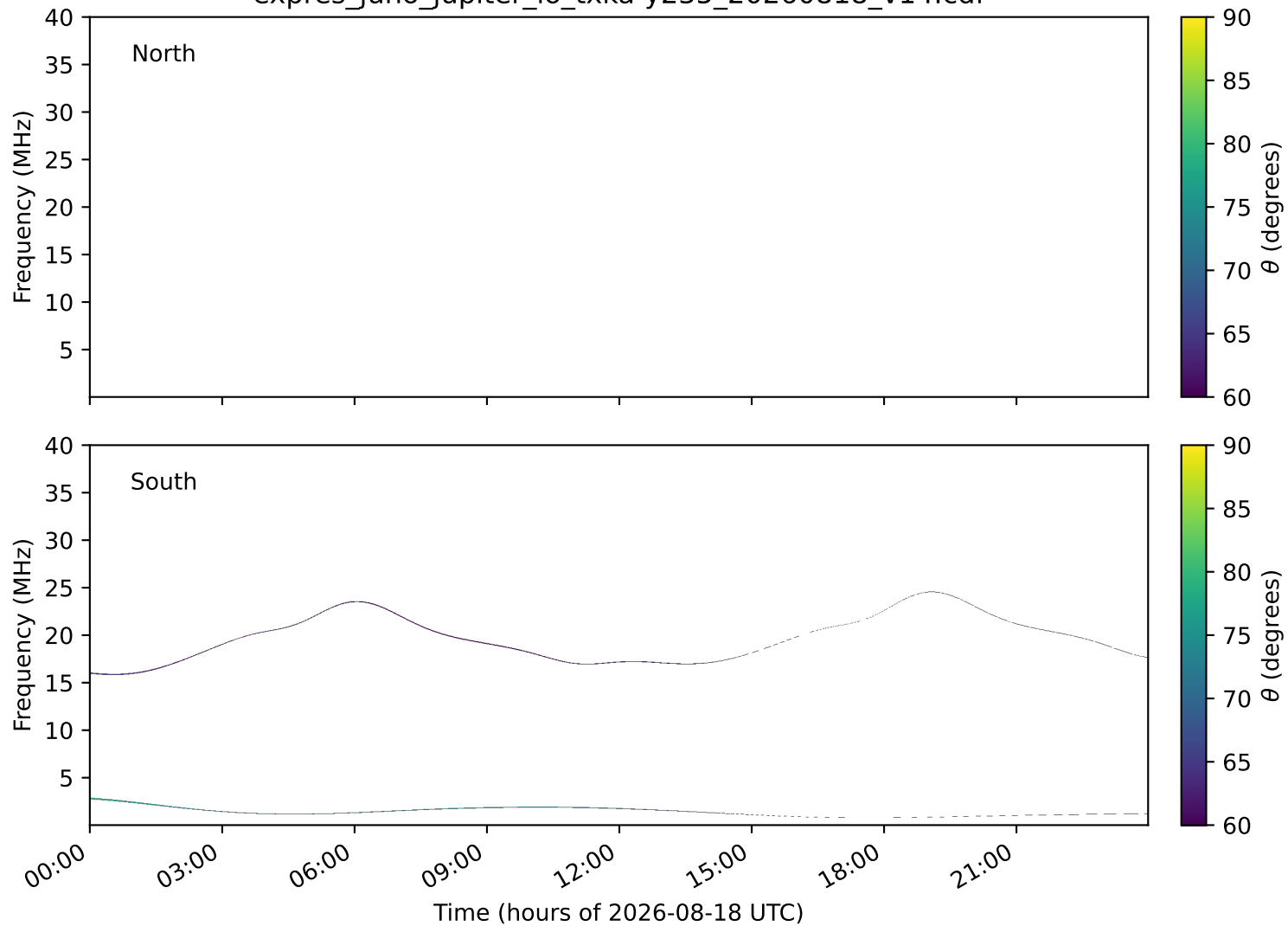
expres_juno_jupiter_io_txka-y235_20260818_v14.cdf
