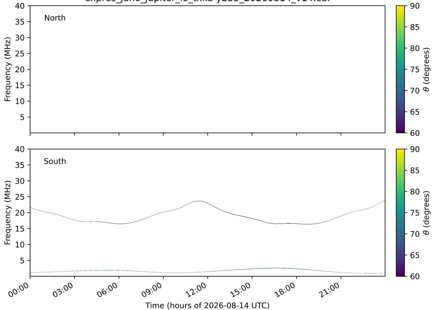
expres_juno_jupiter_io_txka-y235_20260814_v14.cdf
