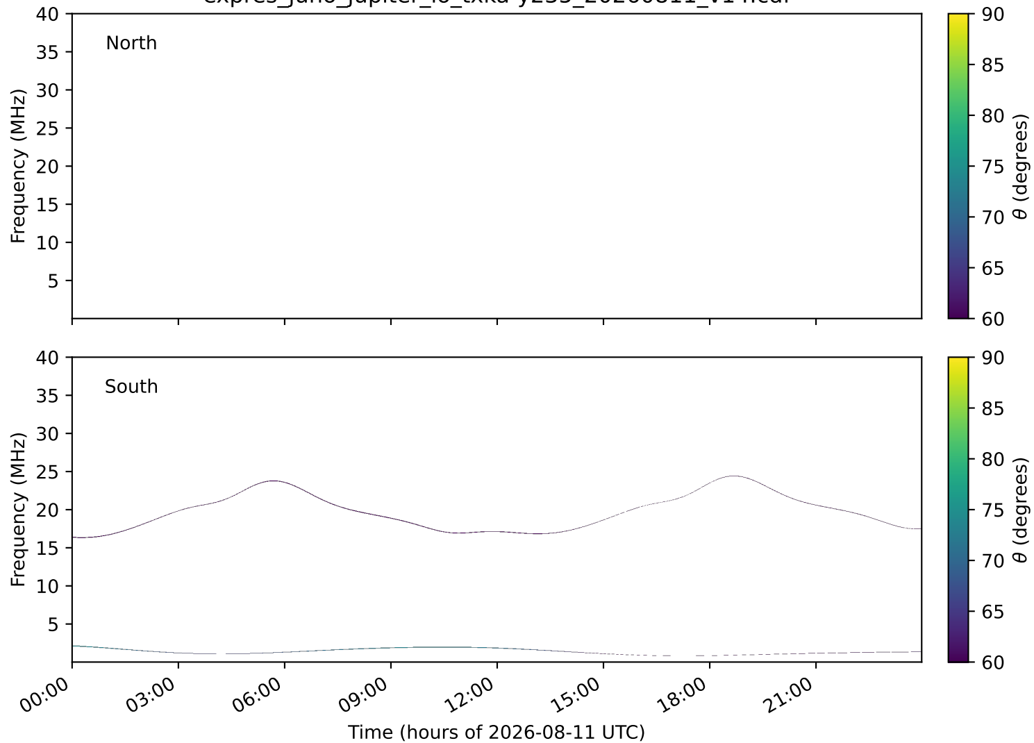
expres_juno_jupiter_io_txka-y235_20260811_v14.cdf
