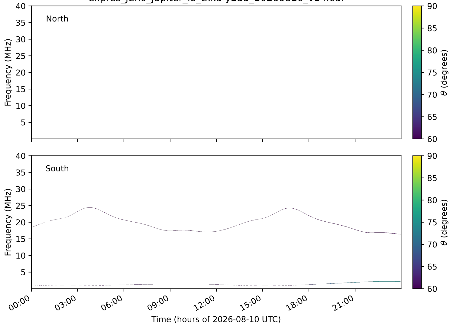
expres_juno_jupiter_io_txka-y235_20260810_v14.cdf
