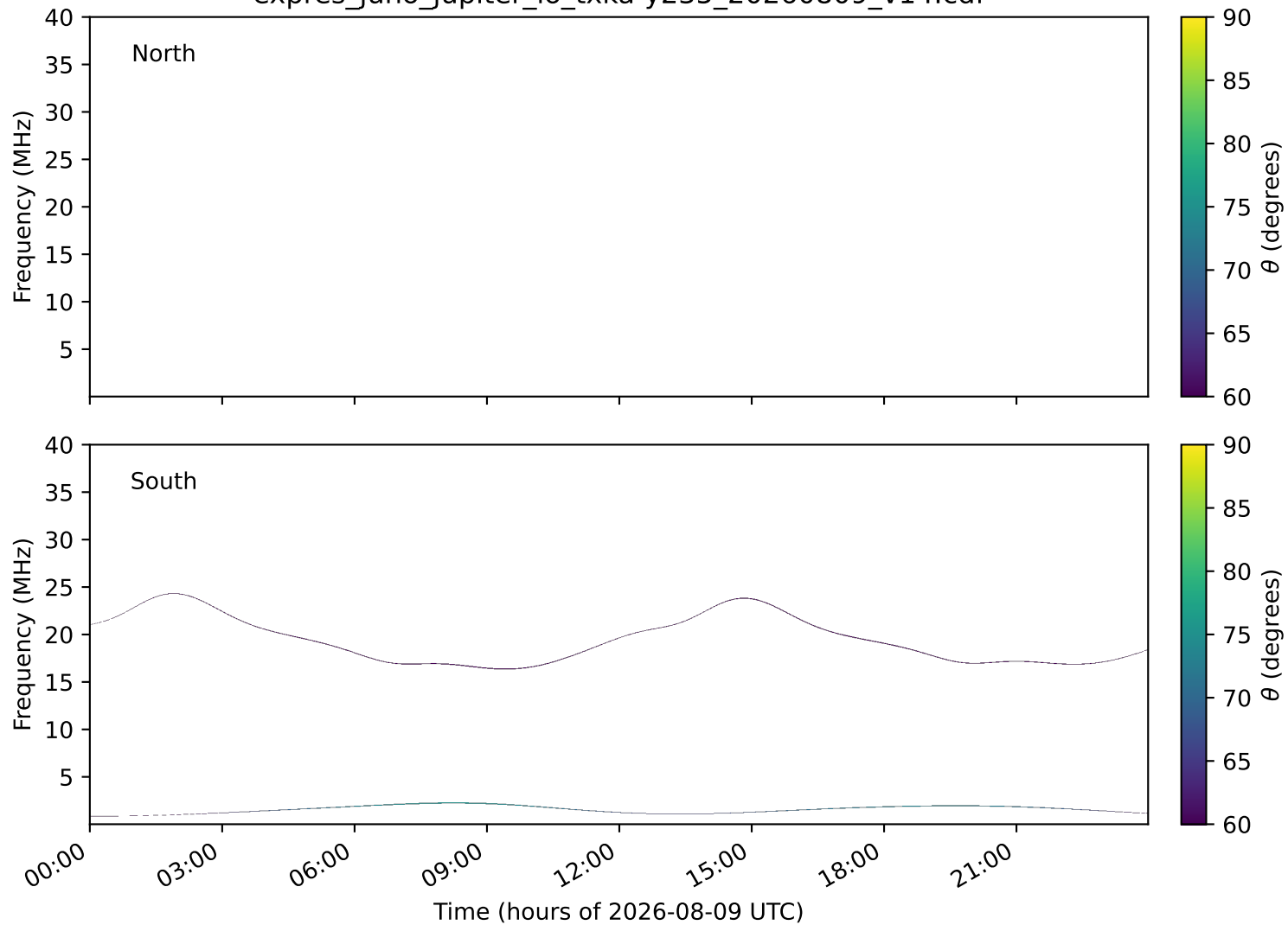
expres_juno_jupiter_io_txka-y235_20260809_v14.cdf
