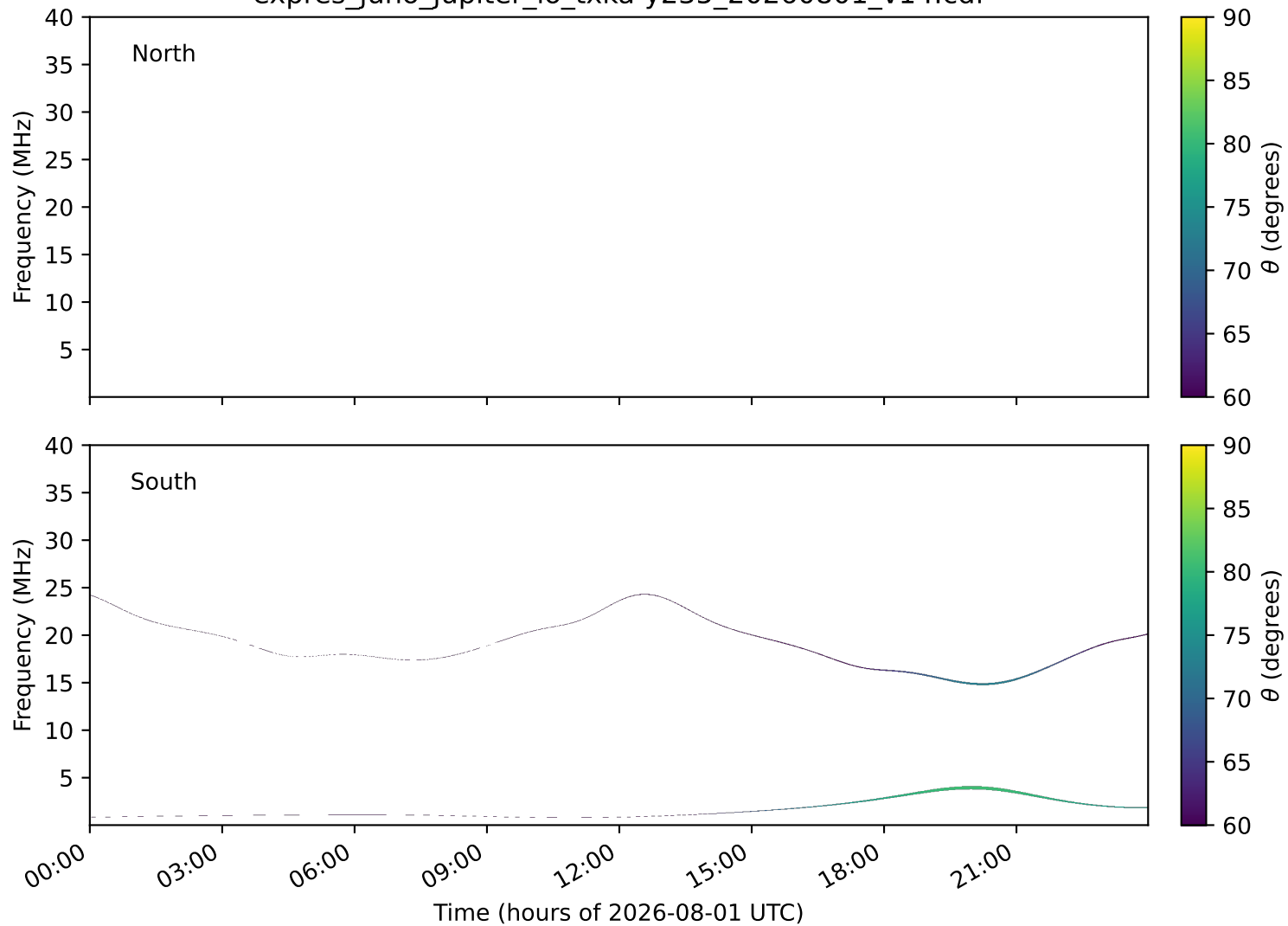
expres_juno_jupiter_io_txka-y235_20260801_v14.cdf
