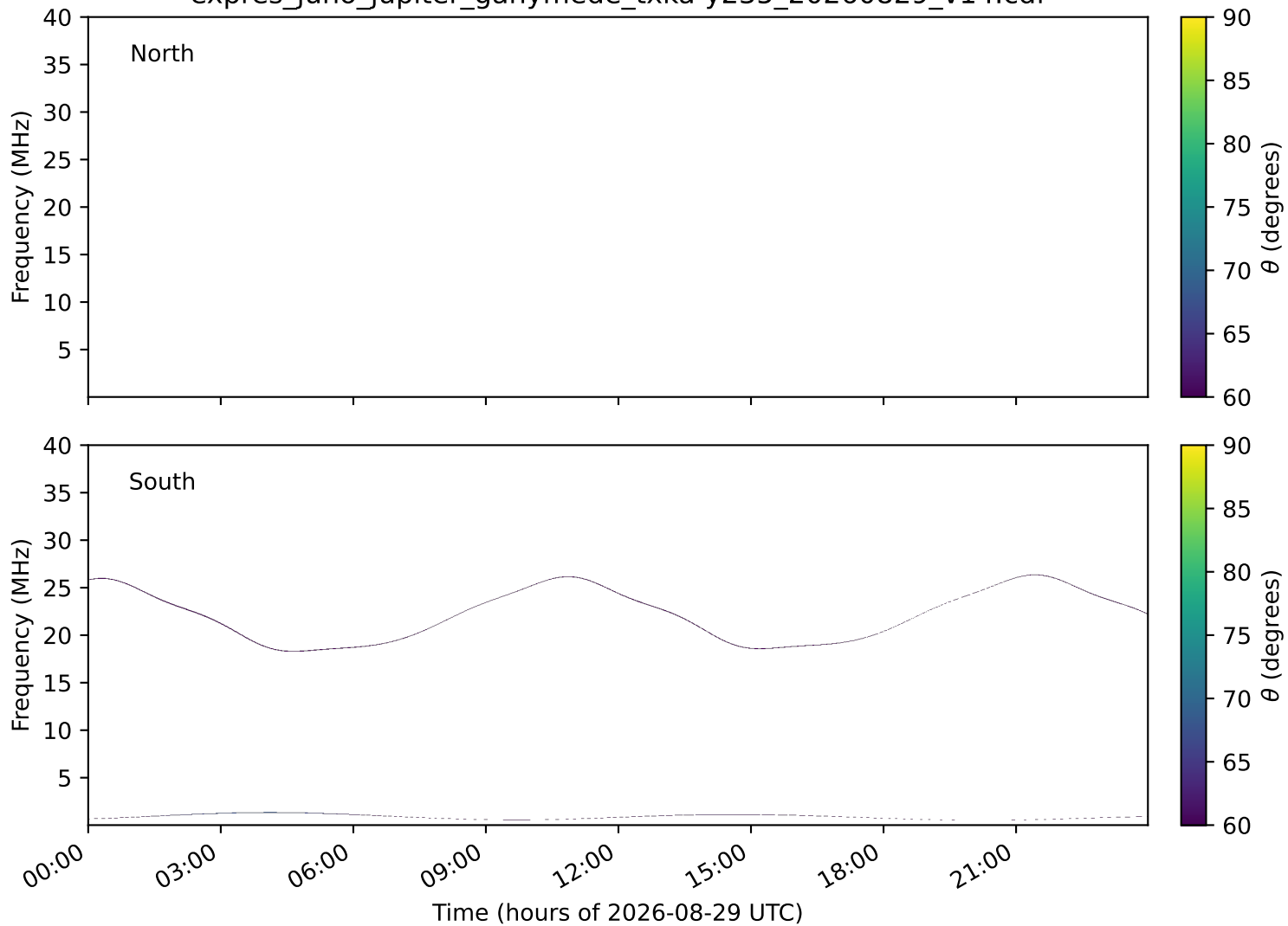
expres_juno_jupiter_ganymede_txka-y235_20260829_v14.cdf
