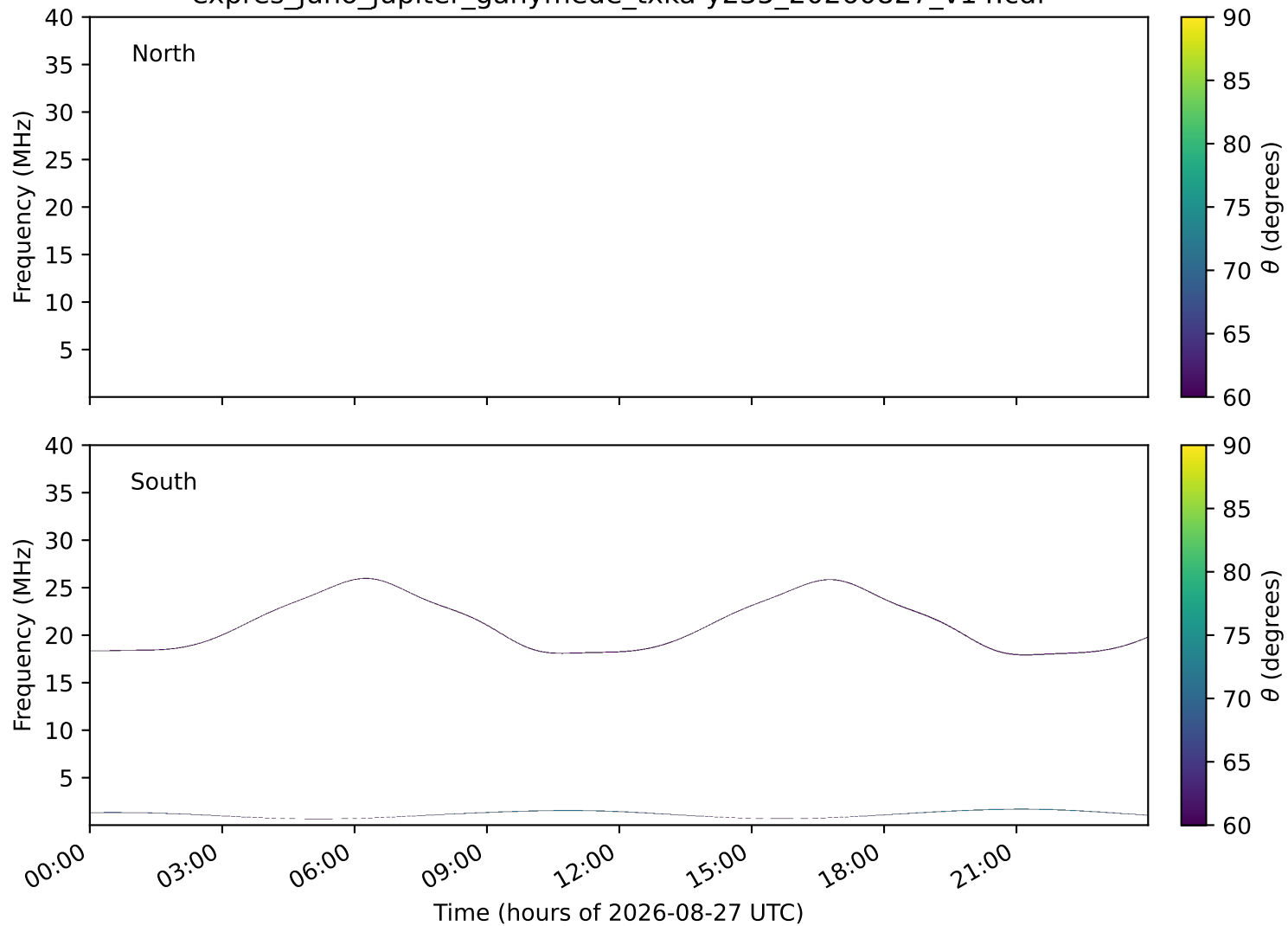
expres_juno_jupiter_ganymede_txka-y235_20260827_v14.cdf
