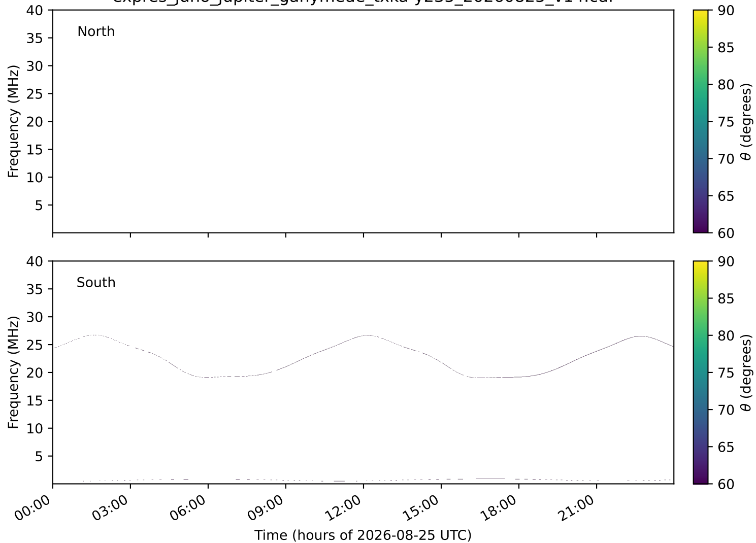
expres_juno_jupiter_ganymede_txka-y235_20260825_v14.cdf
