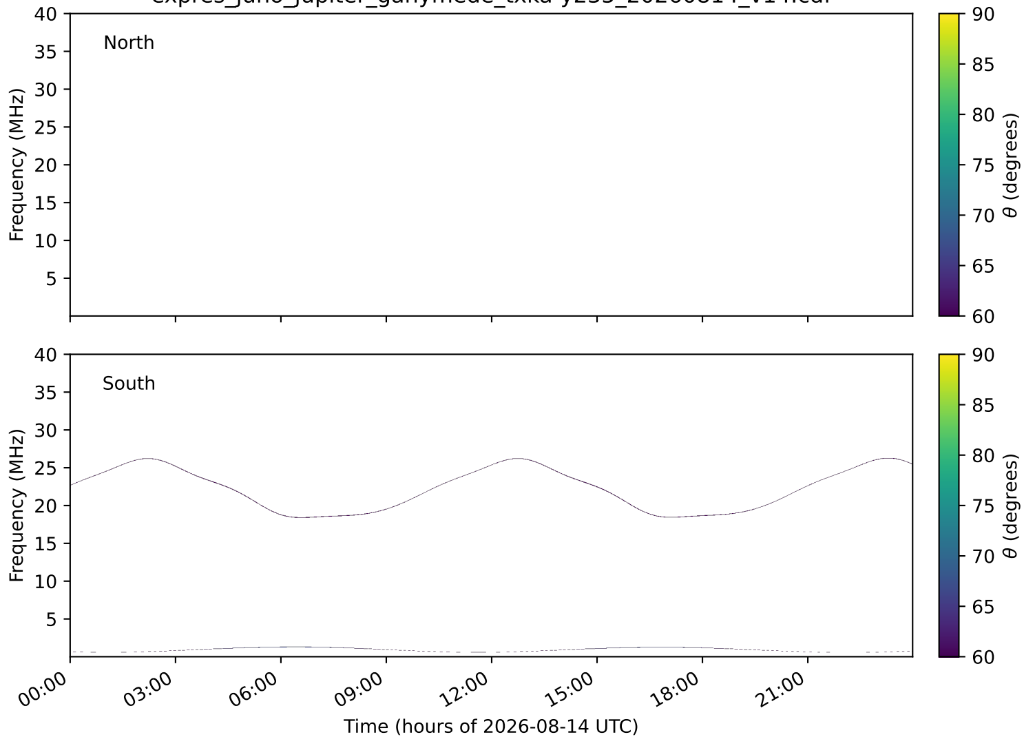
expres_juno_jupiter_ganymede_txka-y235_20260814_v14.cdf
