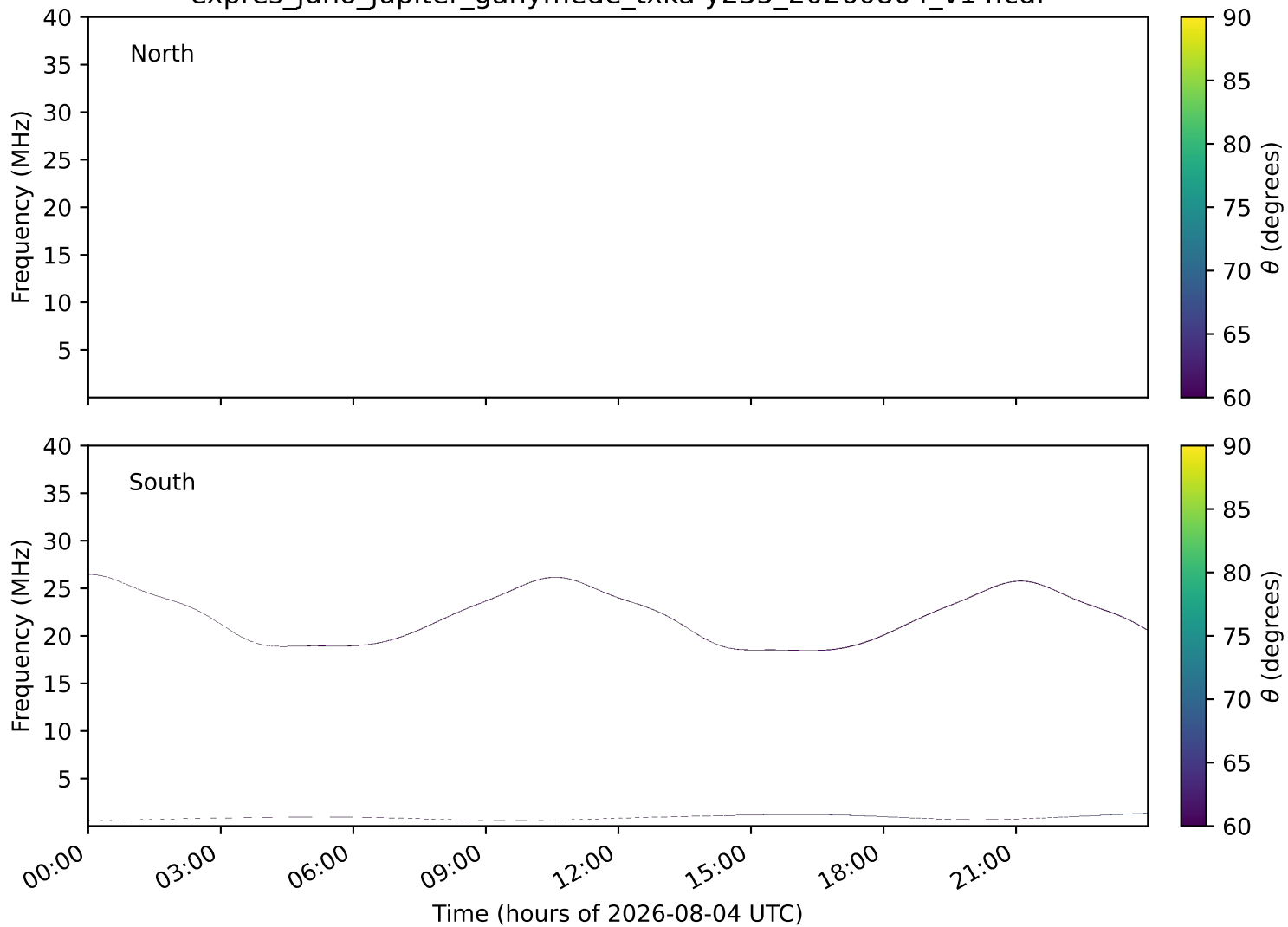
expres_juno_jupiter_ganymede_txka-y235_20260804_v14.cdf
